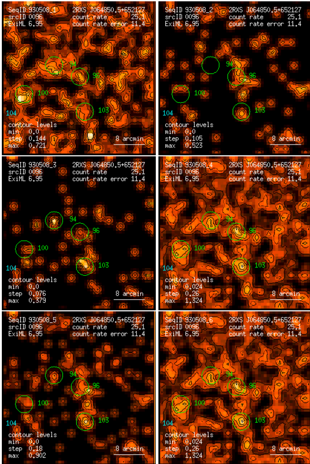
Figure 96: RASS 930508: detection 0096: band rate images, Gaussian filter: (1) PSPC channels 11 – 41, (2) 52 – 90, (3) 91 – 201, (4) 11 – 235, (5) 52 – 201, (6) 11 – 201. Broad band rates in counts/ks. Band rate contour levels in counts/ks/arcmin 2 .
