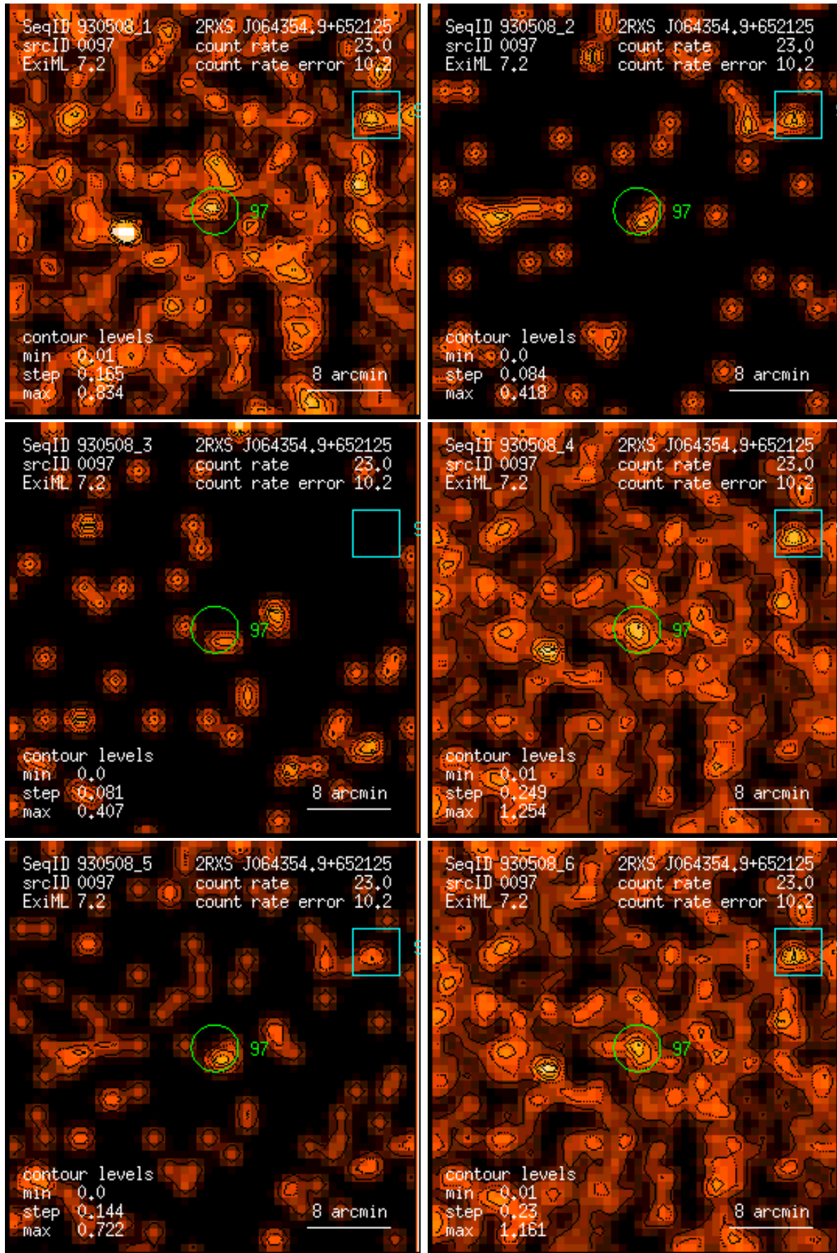
Figure 97: RASS 930508: detection 0097: band rate images, Gaussian filter: (1) PSPC channels 11 – 41, (2) 52 – 90, (3) 91 – 201, (4) 11 – 235, (5) 52 – 201, (6) 11 – 201. Broad band rates in counts/ks. Band rate contour levels in counts/ks/arcmin 2 .
