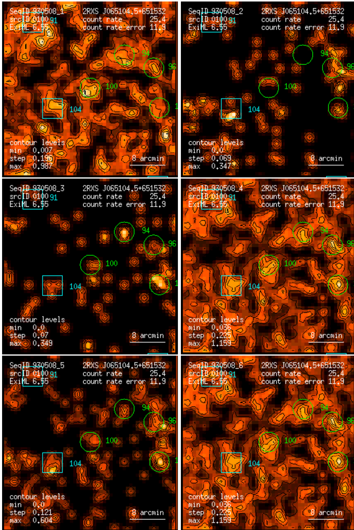
Figure 100: RASS 930508: detection 0100: band rate images, Gaussian filter: (1) PSPC channels 11 – 41, (2) 52 – 90, (3) 91 – 201, (4) 11 – 235, (5) 52 – 201, (6) 11 – 201. Broad band rates in counts/ks. Band rate contour levels in counts/ks/arcmin 2 .
