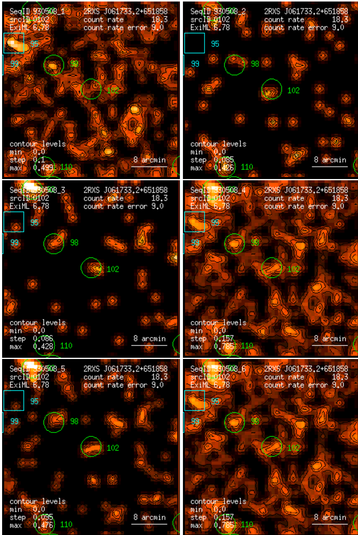
Figure 102: RASS 930508: detection 0102: band rate images, Gaussian filter: (1) PSPC channels 11 – 41, (2) 52 – 90, (3) 91 – 201, (4) 11 – 235, (5) 52 – 201, (6) 11 – 201. Broad band rates in counts/ks. Band rate contour levels in counts/ks/arcmin 2 .
