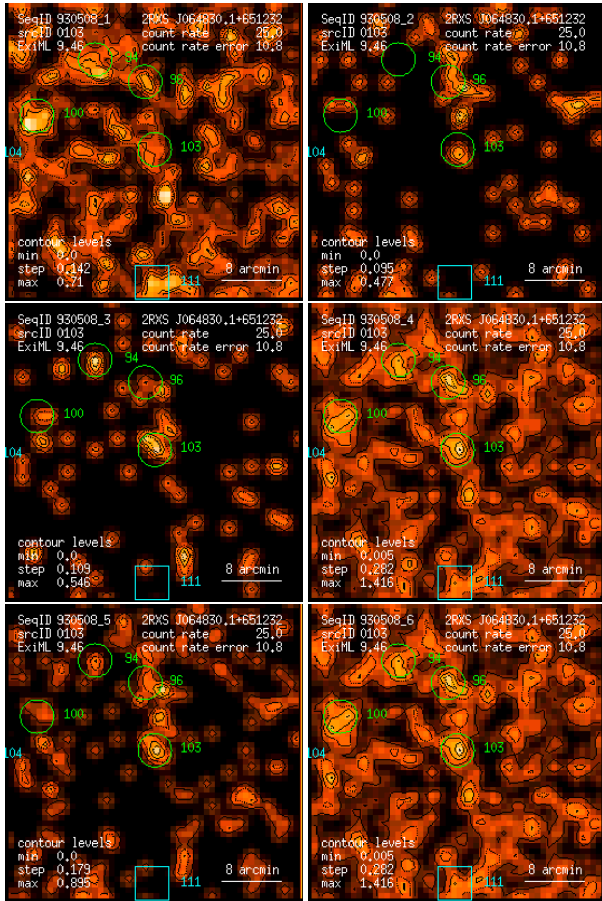
Figure 103: RASS 930508: detection 0103: band rate images, Gaussian filter: (1) PSPC channels 11 – 41, (2) 52 – 90, (3) 91 – 201, (4) 11 – 235, (5) 52 – 201, (6) 11 – 201. Broad band rates in counts/ks. Band rate contour levels in counts/ks/arcmin 2 .
