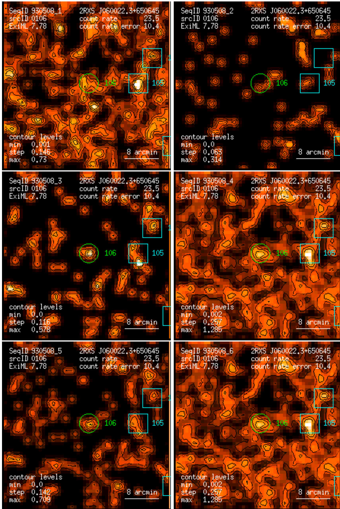
Figure 106: RASS 930508: detection 0106: band rate images, Gaussian filter: (1) PSPC channels 11 – 41, (2) 52 – 90, (3) 91 – 201, (4) 11 – 235, (5) 52 – 201, (6) 11 – 201. Broad band rates in counts/ks. Band rate contour levels in counts/ks/arcmin 2 .
