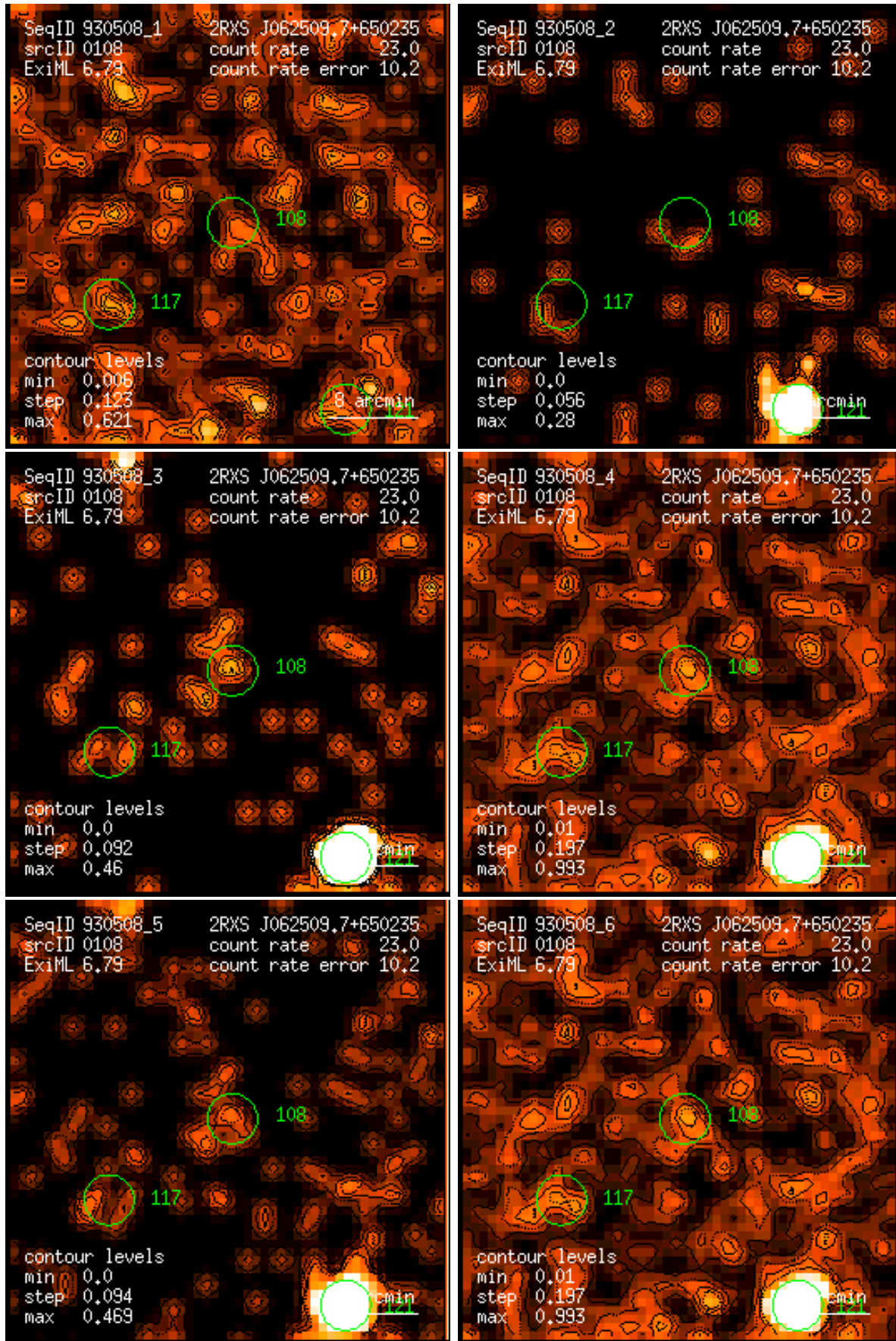
Figure 108: RASS 930508: detection 0108: band rate images, Gaussian filter: (1) PSPC channels 11 – 41, (2) 52 – 90, (3) 91 – 201, (4) 11 – 235, (5) 52 – 201, (6) 11 – 201. Broad band rates in counts/ks. Band rate contour levels in counts/ks/arcmin 2 .
