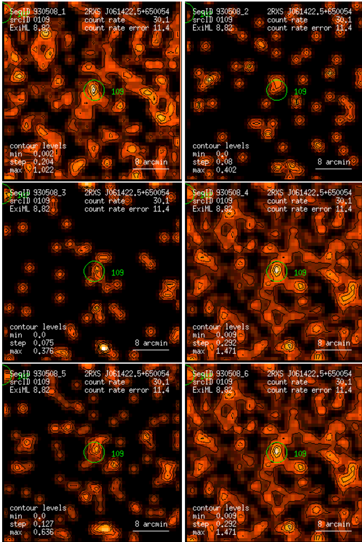
Figure 109: RASS 930508: detection 0109: band rate images, Gaussian filter: (1) PSPC channels 11 – 41, (2) 52 – 90, (3) 91 – 201, (4) 11 – 235, (5) 52 – 201, (6) 11 – 201. Broad band rates in counts/ks. Band rate contour levels in counts/ks/arcmin 2 .
