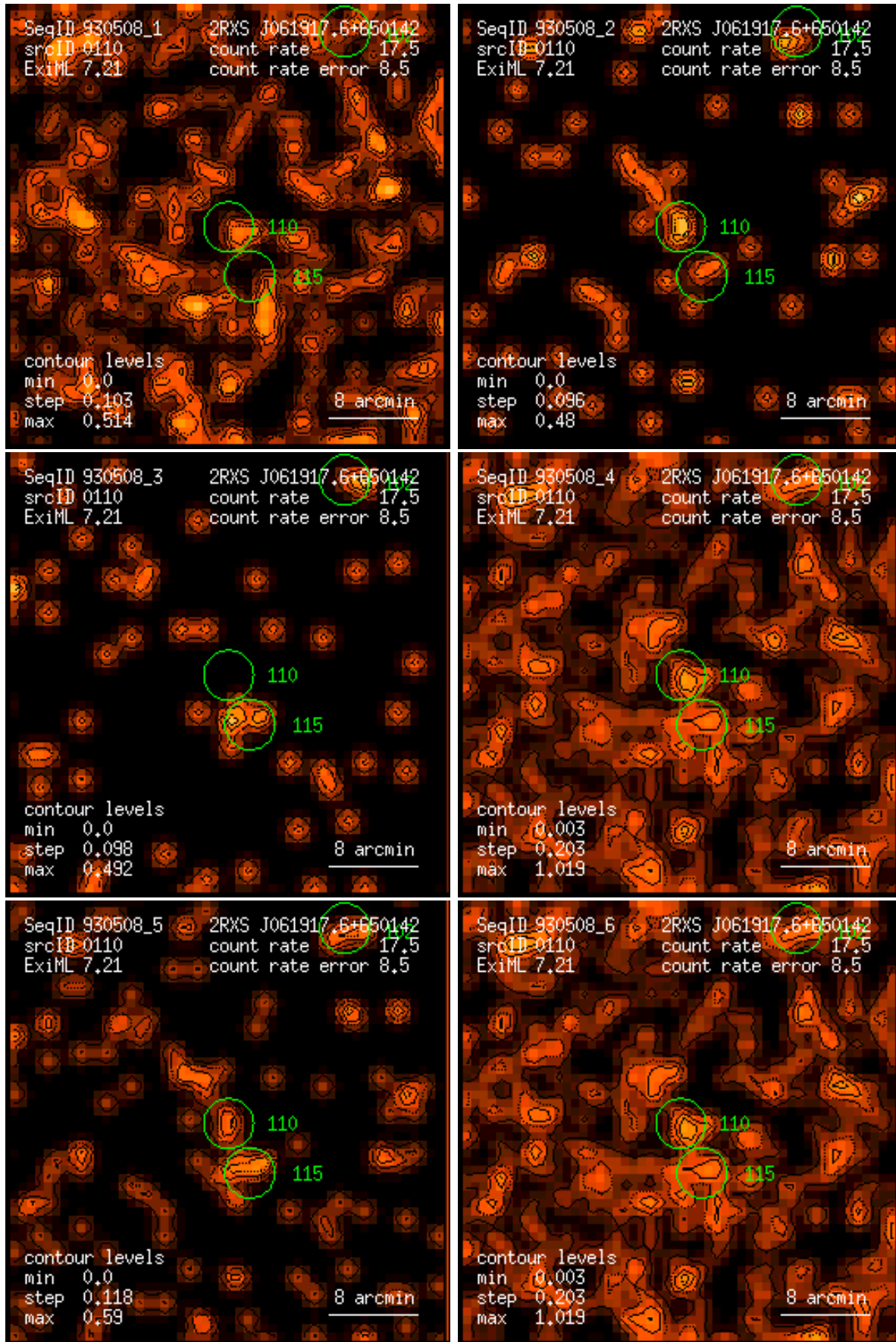
Figure 110: RASS 930508: detection 0110: band rate images, Gaussian filter: (1) PSPC channels 11 – 41, (2) 52 – 90, (3) 91 – 201, (4) 11 – 235, (5) 52 – 201, (6) 11 – 201. Broad band rates in counts/ks. Band rate contour levels in counts/ks/arcmin 2 .
