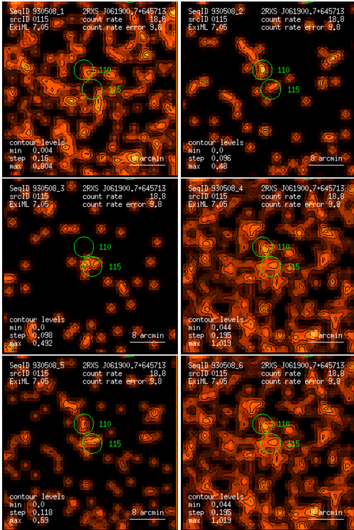
Figure 115: RASS 930508: detection 0115: band rate images, Gaussian filter: (1) PSPC channels 11 – 41, (2) 52 – 90, (3) 91 – 201, (4) 11 – 235, (5) 52 – 201, (6) 11 – 201. Broad band rates in counts/ks. Band rate contour levels in counts/ks/arcmin 2 .
