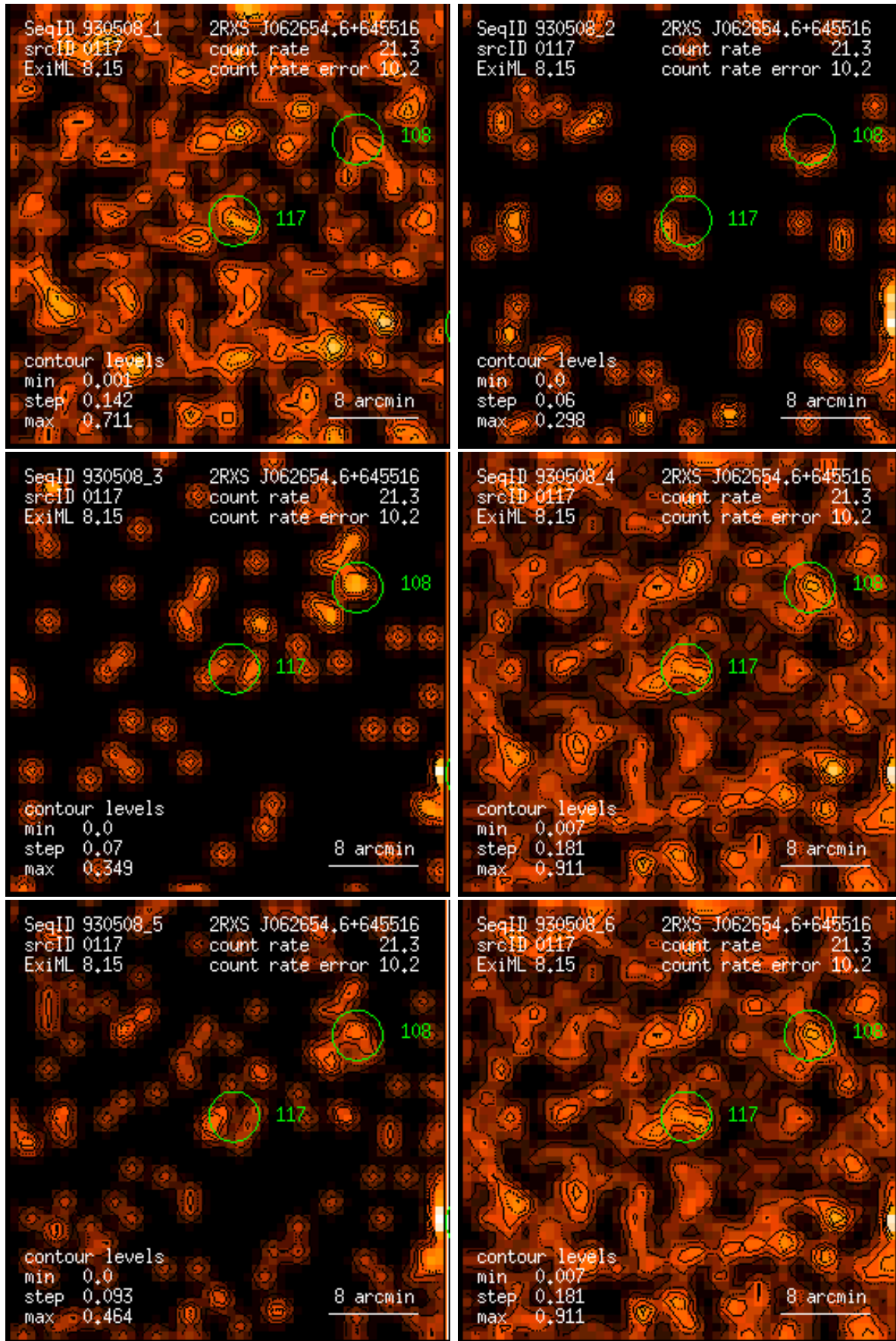
Figure 117: RASS 930508: detection 0117: band rate images, Gaussian filter: (1) PSPC channels 11 – 41, (2) 52 – 90, (3) 91 – 201, (4) 11 – 235, (5) 52 – 201, (6) 11 – 201. Broad band rates in counts/ks. Band rate contour levels in counts/ks/arcmin 2 .
