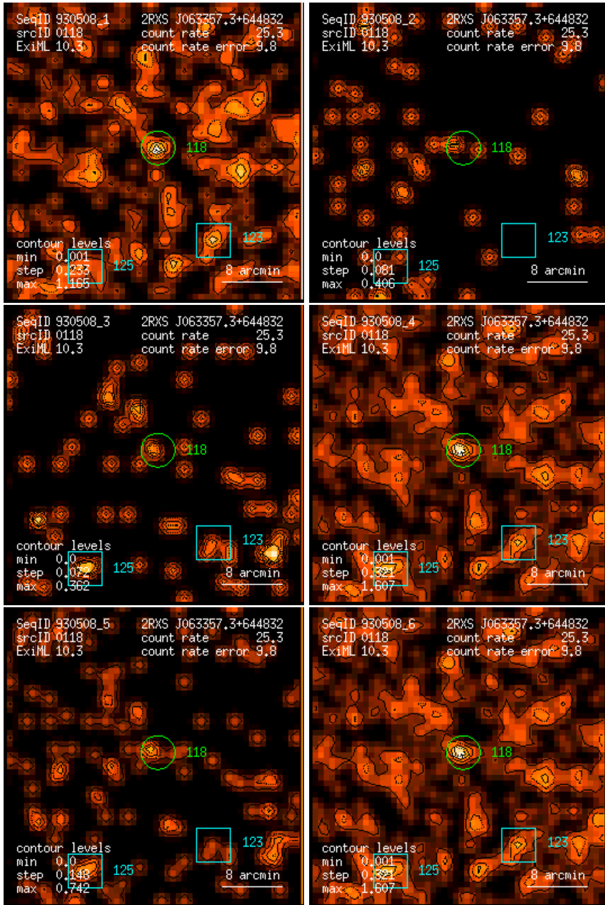
Figure 118: RASS 930508: detection 0118: band rate images, Gaussian filter: (1) PSPC channels 11 – 41, (2) 52 – 90, (3) 91 – 201, (4) 11 – 235, (5) 52 – 201, (6) 11 – 201. Broad band rates in counts/ks. Band rate contour levels in counts/ks/arcmin 2 .
