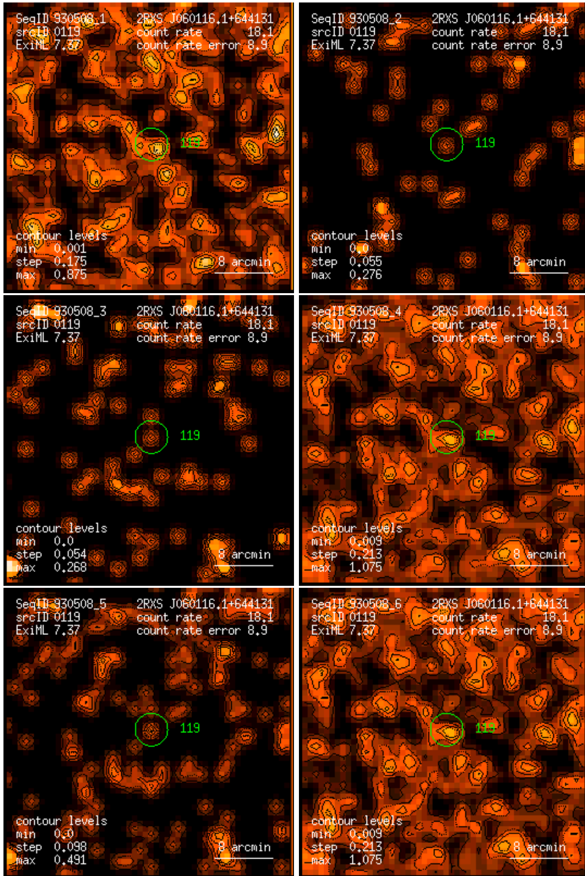
Figure 119: RASS 930508: detection 0119: band rate images, Gaussian filter: (1) PSPC channels 11 – 41, (2) 52 – 90, (3) 91 – 201, (4) 11 – 235, (5) 52 – 201, (6) 11 – 201. Broad band rates in counts/ks. Band rate contour levels in counts/ks/arcmin 2 .
