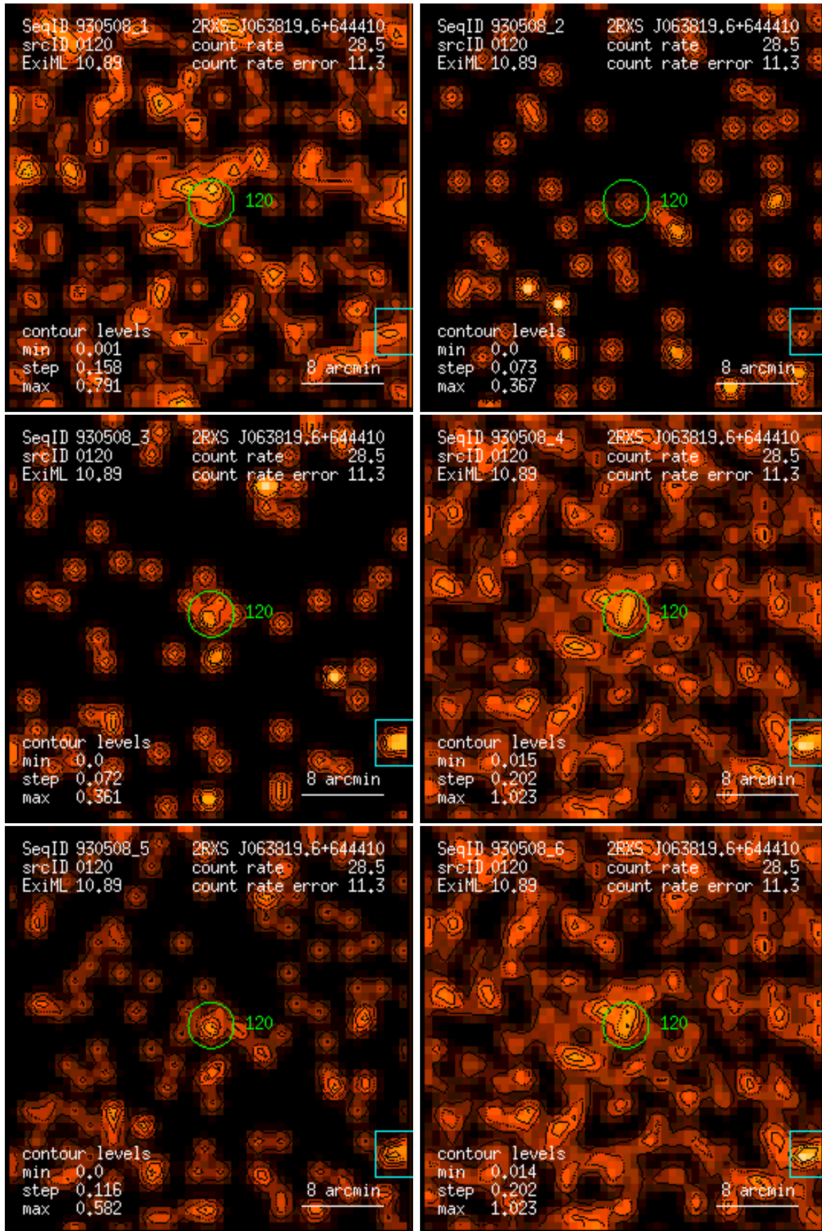
Figure 120: RASS 930508: detection 0120: band rate images, Gaussian filter: (1) PSPC channels 11 – 41, (2) 52 – 90, (3) 91 – 201, (4) 11 – 235, (5) 52 – 201, (6) 11 – 201. Broad band rates in counts/ks. Band rate contour levels in counts/ks/arcmin 2 .
