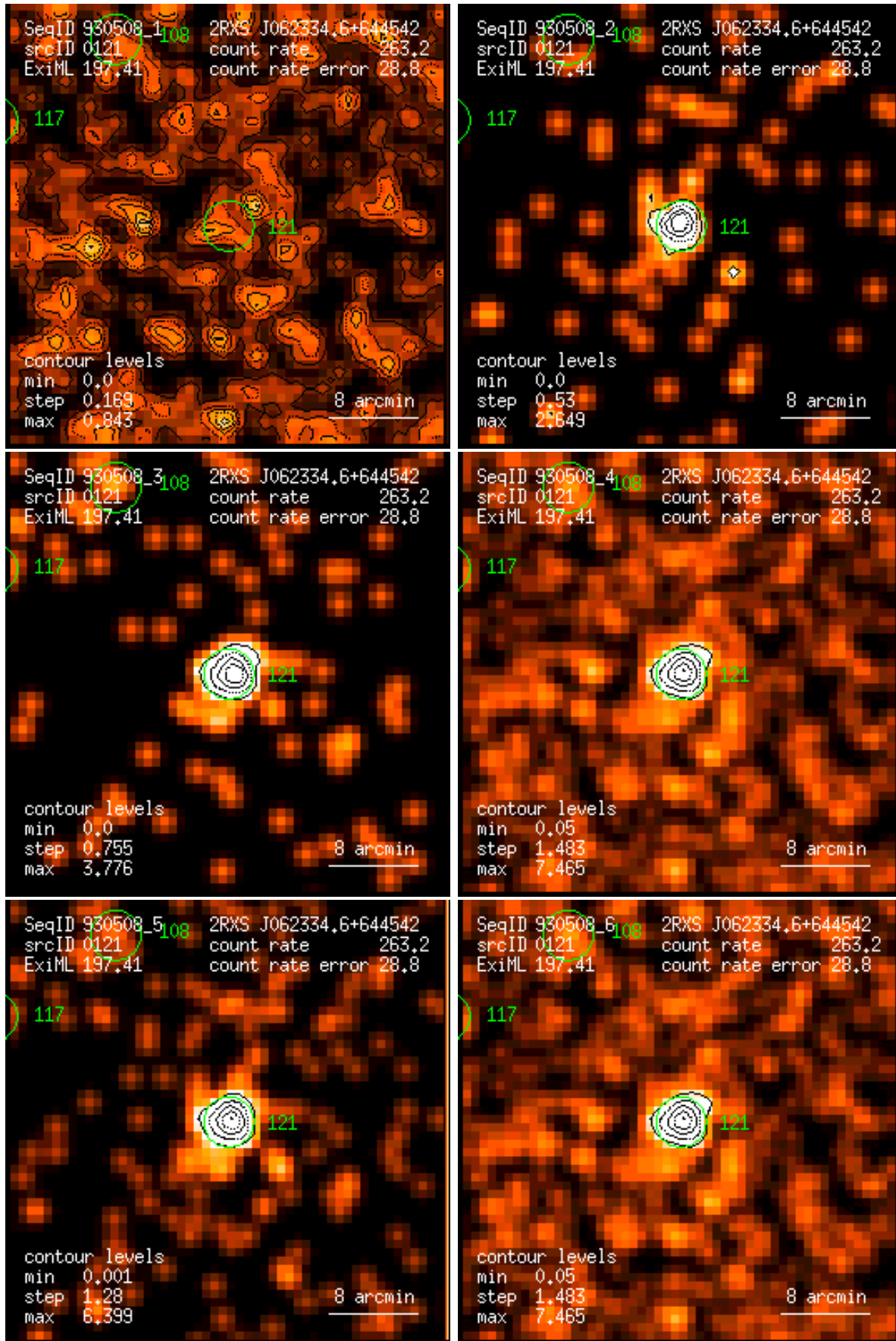
Figure 121: RASS 930508: detection 0121: band rate images, Gaussian filter: (1) PSPC channels 11 – 41, (2) 52 – 90, (3) 91 – 201, (4) 11 – 235, (5) 52 – 201, (6) 11 – 201. Broad band rates in counts/ks. Band rate contour levels in counts/ks/arcmin 2 .
