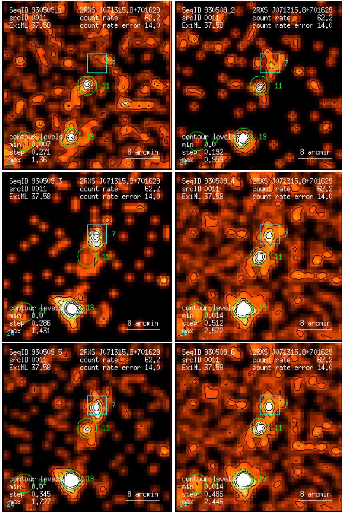
Figure 11: RASS 930509: detection 0011: band rate images, Gaussian filter: (1) PSPC channels 11 – 41, (2) 52 – 90, (3) 91 – 201, (4) 11 – 235, (5) 52 – 201, (6) 11 – 201. Broad band rates in counts/ks. Band rate contour levels in counts/ks/arcmin 2 .
