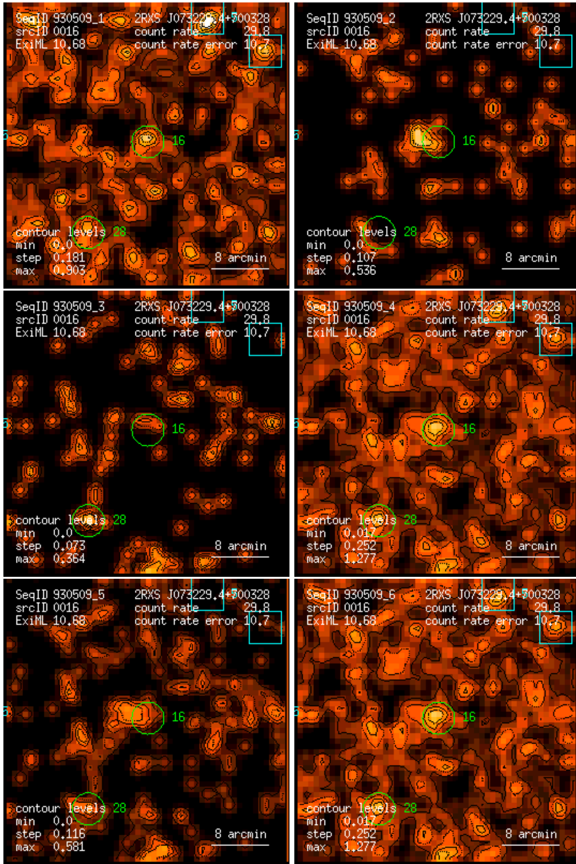
Figure 16: RASS 930509: detection 0016: band rate images, Gaussian filter: (1) PSPC channels 11 – 41, (2) 52 – 90, (3) 91 – 201, (4) 11 – 235, (5) 52 – 201, (6) 11 – 201. Broad band rates in counts/ks. Band rate contour levels in counts/ks/arcmin 2 .
