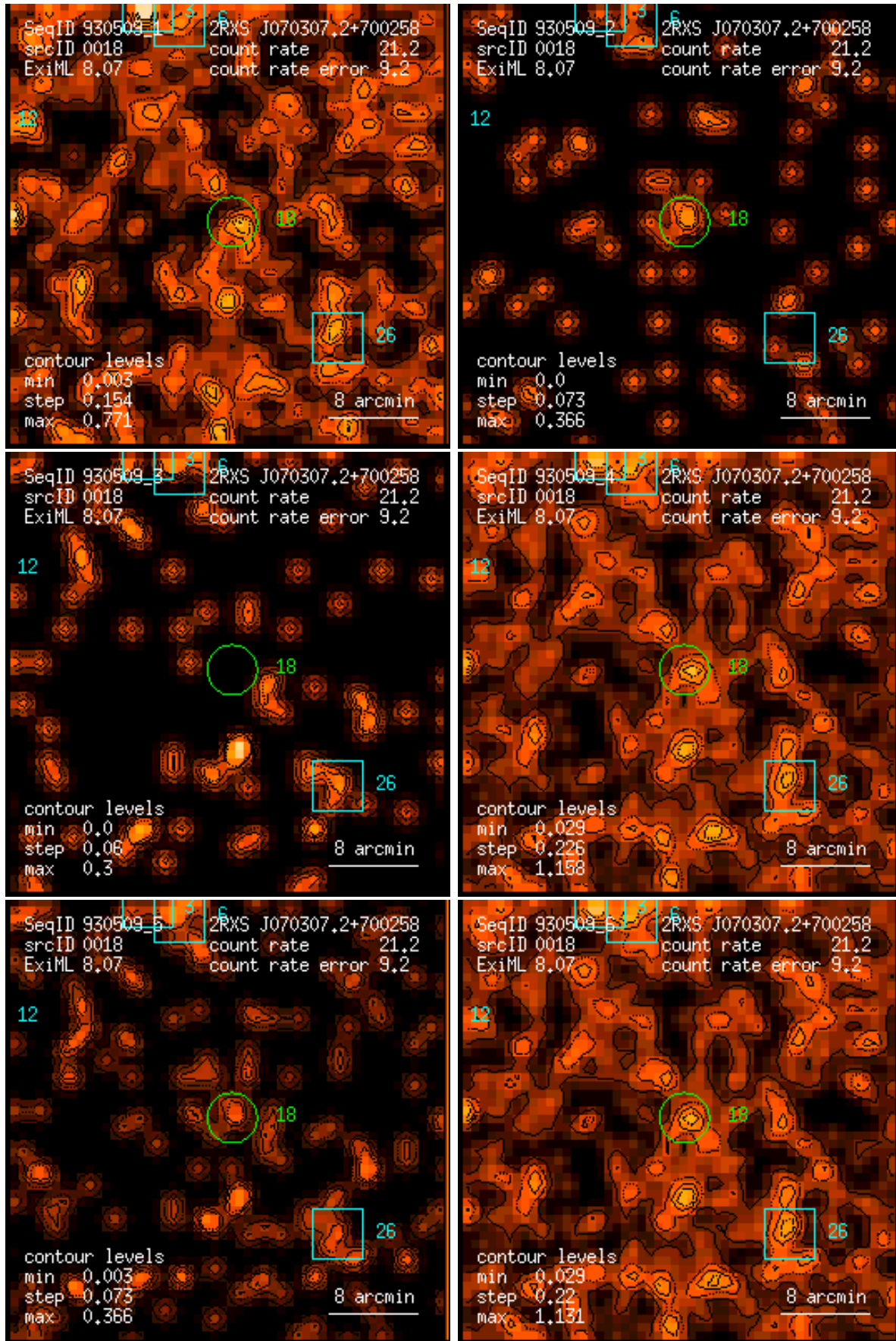
Figure 18: RASS 930509: detection 0018: band rate images, Gaussian filter: (1) PSPC channels 11 – 41, (2) 52 – 90, (3) 91 – 201, (4) 11 – 235, (5) 52 – 201, (6) 11 – 201. Broad band rates in counts/ks. Band rate contour levels in counts/ks/arcmin 2 .
