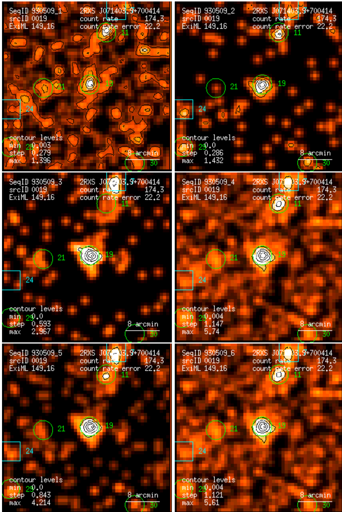
Figure 19: RASS 930509: detection 0019: band rate images, Gaussian filter: (1) PSPC channels 11 – 41, (2) 52 – 90, (3) 91 – 201, (4) 11 – 235, (5) 52 – 201, (6) 11 – 201. Broad band rates in counts/ks. Band rate contour levels in counts/ks/arcmin 2 .
