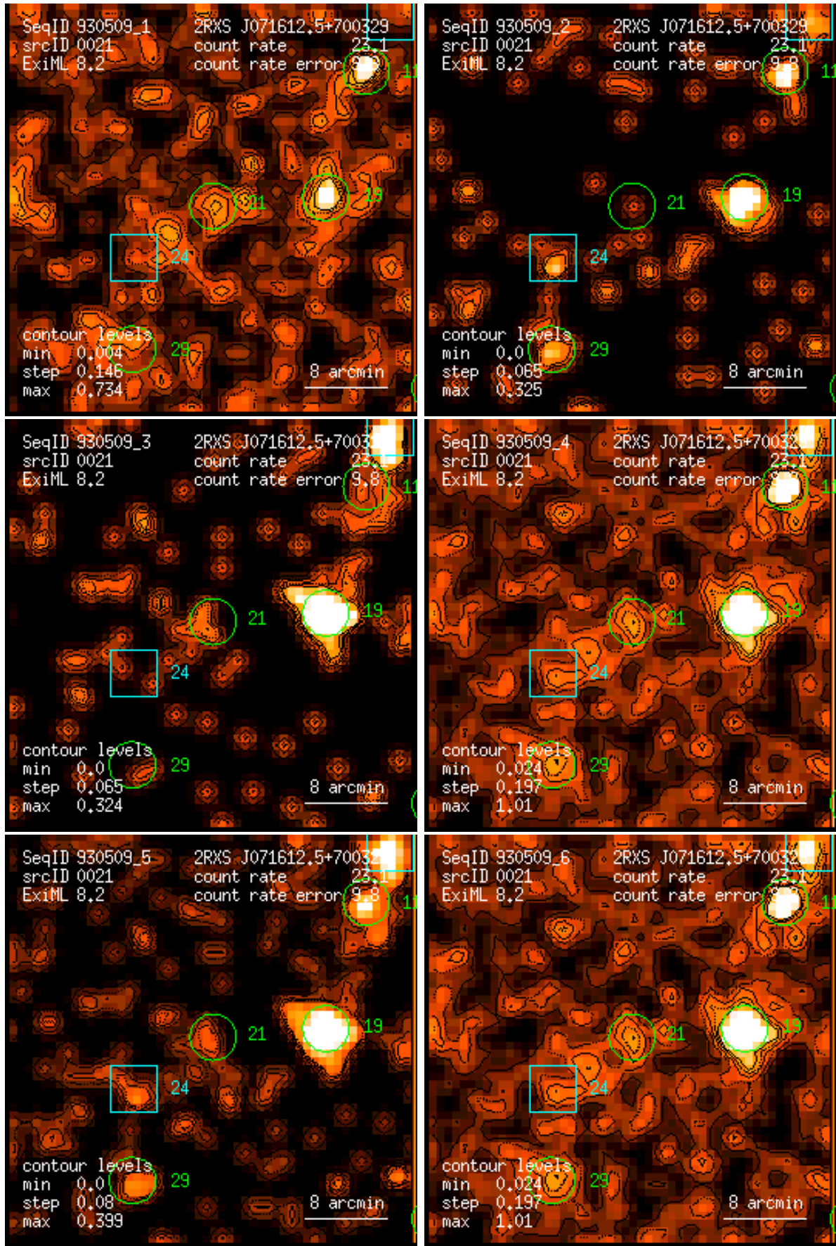
Figure 21: RASS 930509: detection 0021: band rate images, Gaussian filter: (1) PSPC channels 11 – 41, (2) 52 – 90, (3) 91 – 201, (4) 11 – 235, (5) 52 – 201, (6) 11 – 201. Broad band rates in counts/ks. Band rate contour levels in counts/ks/arcmin 2 .
