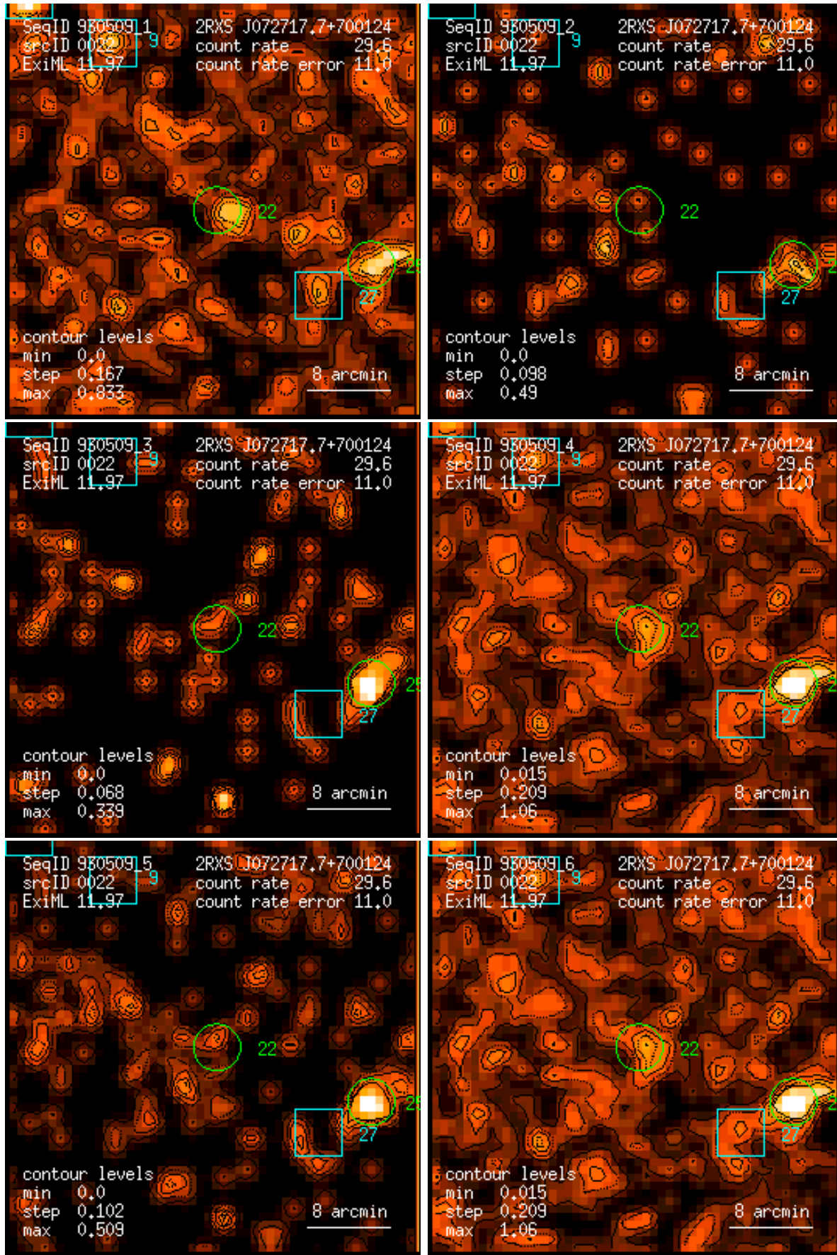
Figure 22: RASS 930509: detection 0022: band rate images, Gaussian filter: (1) PSPC channels 11 – 41, (2) 52 – 90, (3) 91 – 201, (4) 11 – 235, (5) 52 – 201, (6) 11 – 201. Broad band rates in counts/ks. Band rate contour levels in counts/ks/arcmin 2 .
