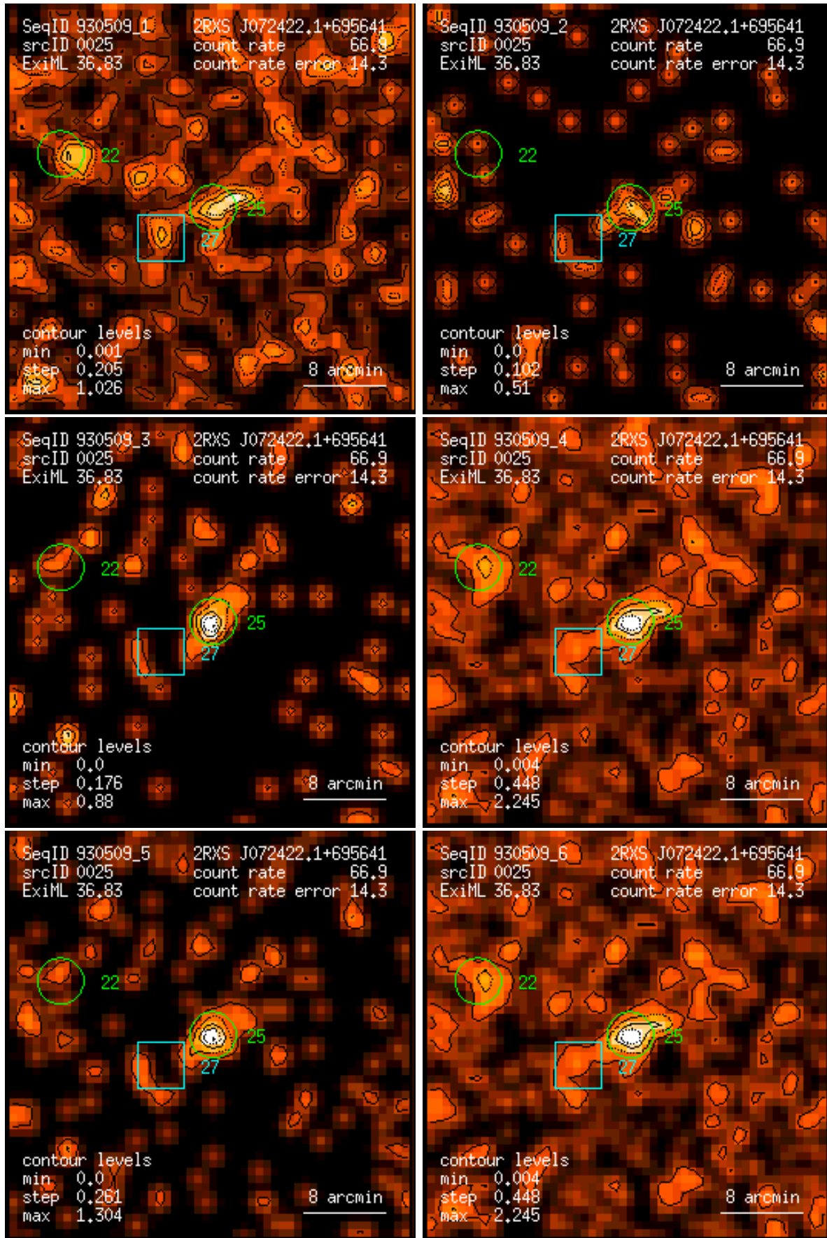
Figure 25: RASS 930509: detection 0025: band rate images, Gaussian filter: (1) PSPC channels 11 – 41, (2) 52 – 90, (3) 91 – 201, (4) 11 – 235, (5) 52 – 201, (6) 11 – 201. Broad band rates in counts/ks. Band rate contour levels in counts/ks/arcmin 2 .
