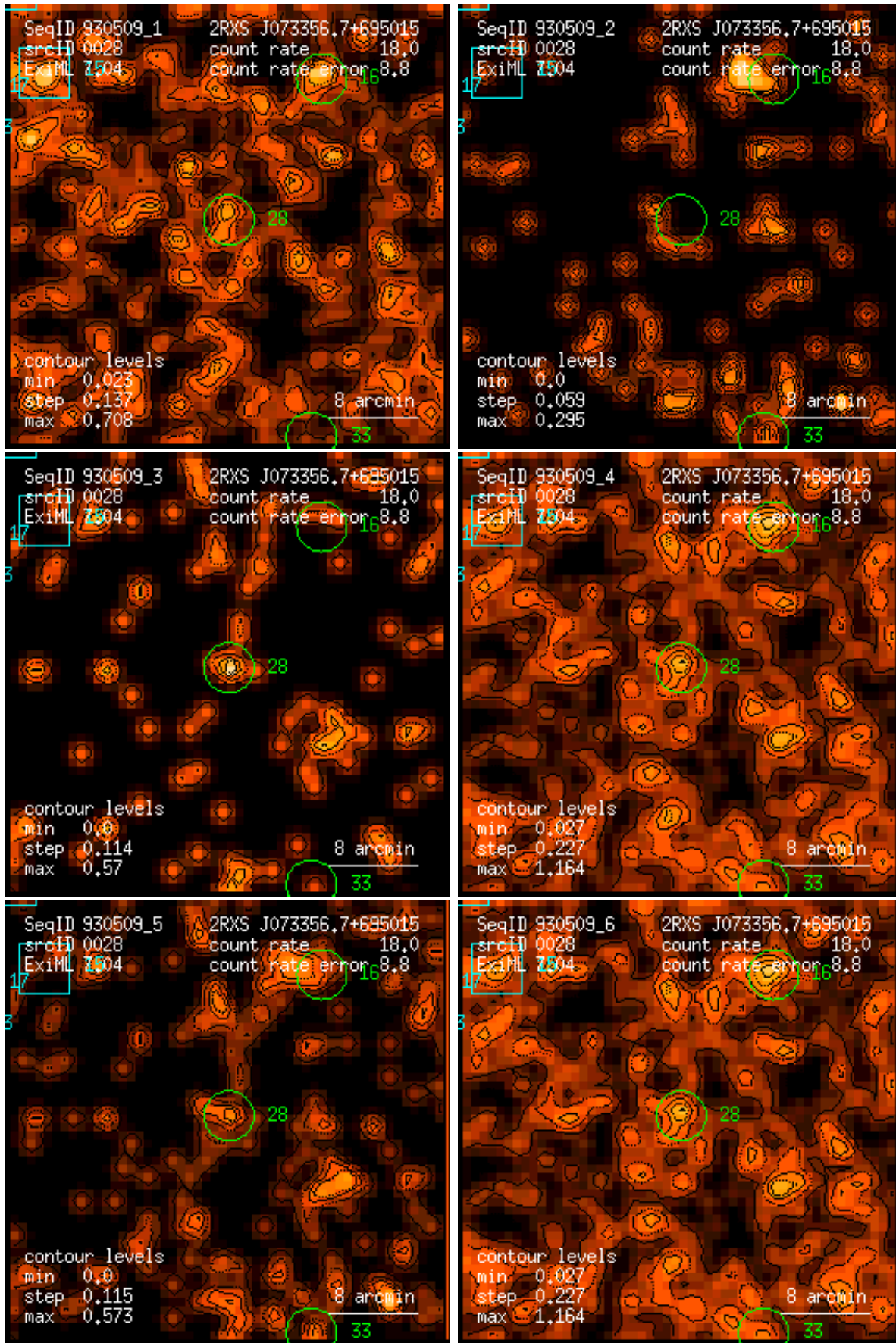
Figure 28: RASS 930509: detection 0028: band rate images, Gaussian filter: (1) PSPC channels 11 – 41, (2) 52 – 90, (3) 91 – 201, (4) 11 – 235, (5) 52 – 201, (6) 11 – 201. Broad band rates in counts/ks. Band rate contour levels in counts/ks/arcmin 2 .
