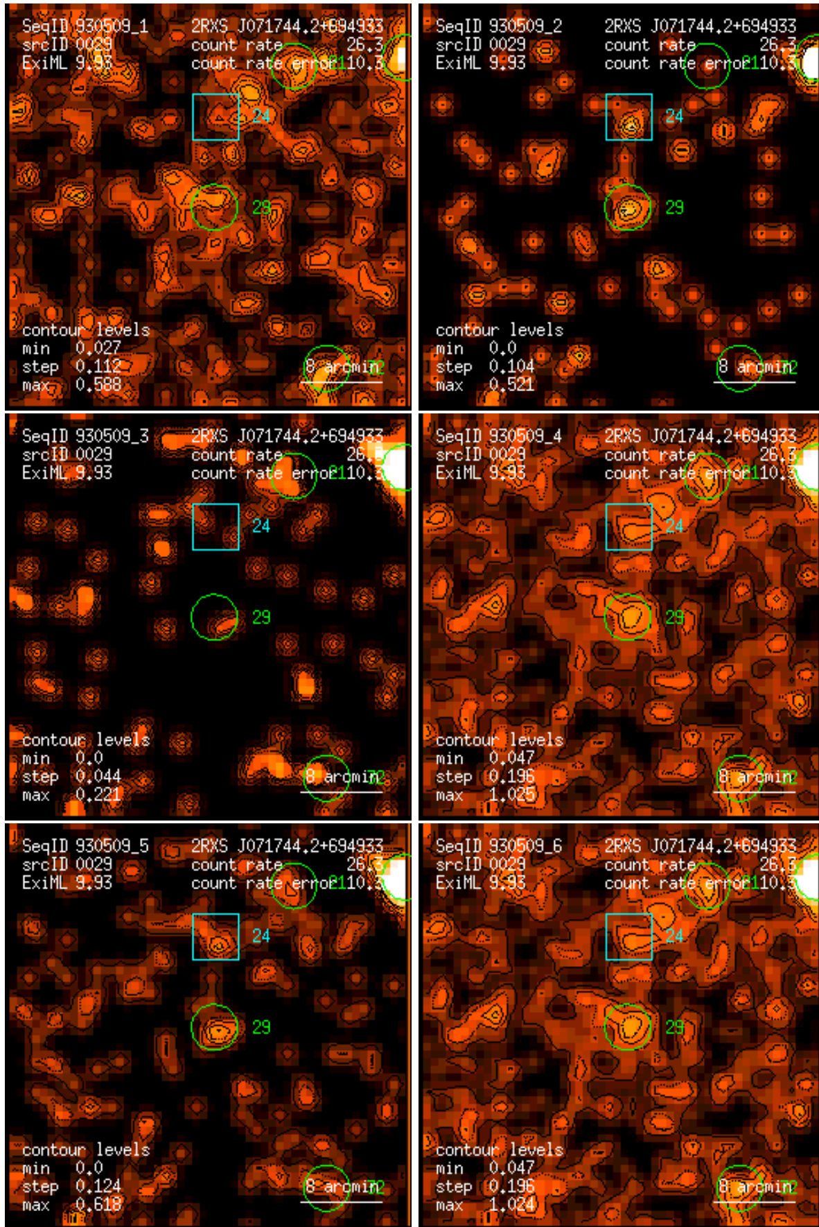
Figure 29: RASS 930509: detection 0029: band rate images, Gaussian filter: (1) PSPC channels 11 – 41, (2) 52 – 90, (3) 91 – 201, (4) 11 – 235, (5) 52 – 201, (6) 11 – 201. Broad band rates in counts/ks. Band rate contour levels in counts/ks/arcmin 2 .
