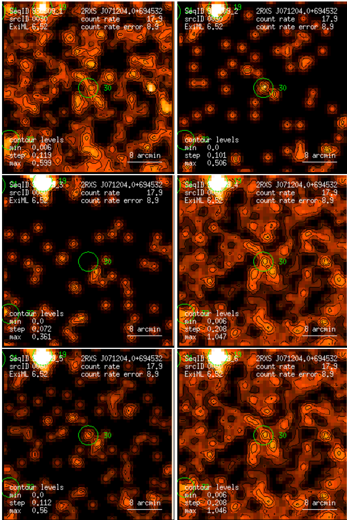
Figure 30: RASS 930509: detection 0030: band rate images, Gaussian filter: (1) PSPC channels 11 – 41, (2) 52 – 90, (3) 91 – 201, (4) 11 – 235, (5) 52 – 201, (6) 11 – 201. Broad band rates in counts/ks. Band rate contour levels in counts/ks/arcmin 2 .
