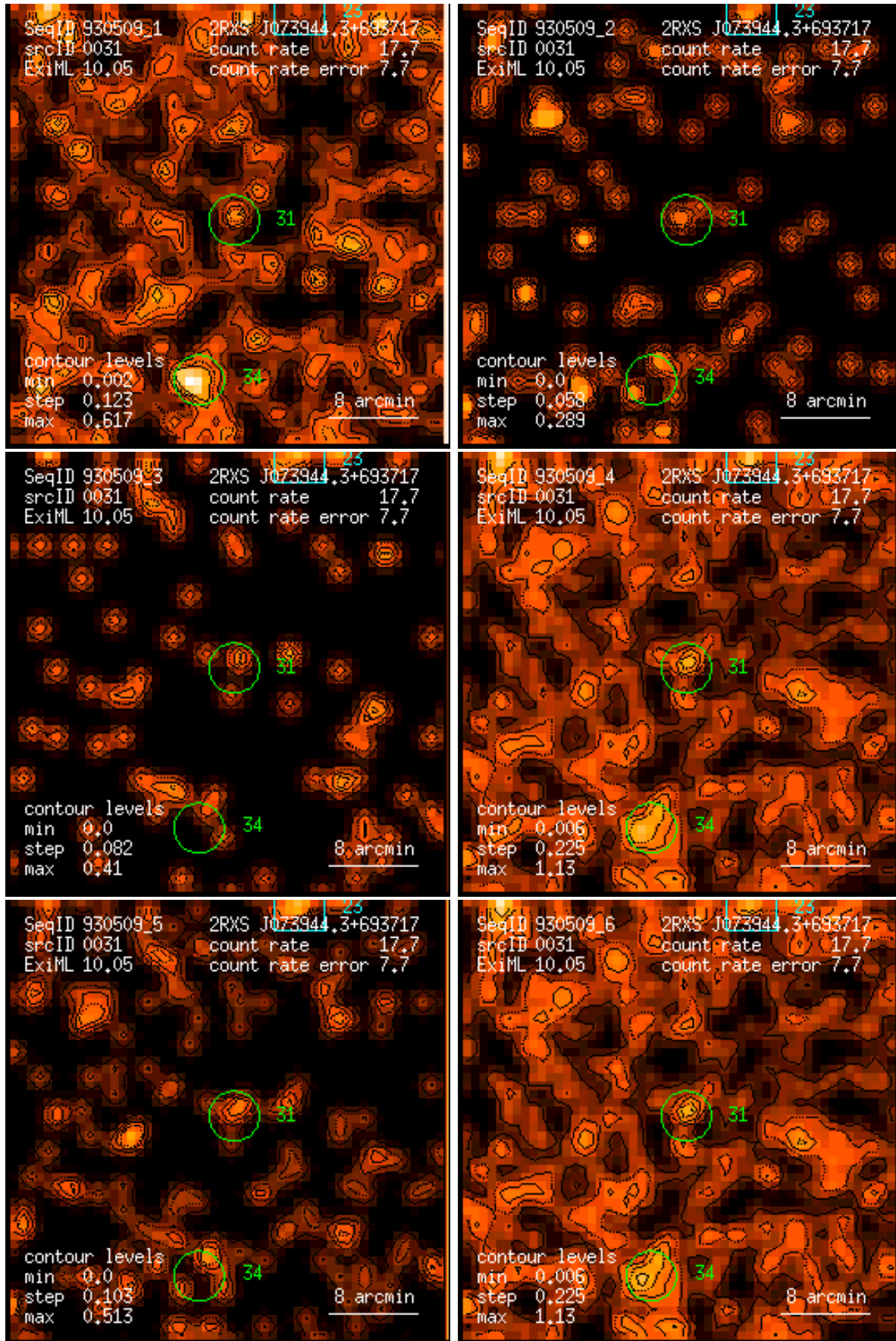
Figure 31: RASS 930509: detection 0031: band rate images, Gaussian filter: (1) PSPC channels 11 – 41, (2) 52 – 90, (3) 91 – 201, (4) 11 – 235, (5) 52 – 201, (6) 11 – 201. Broad band rates in counts/ks. Band rate contour levels in counts/ks/arcmin 2 .
