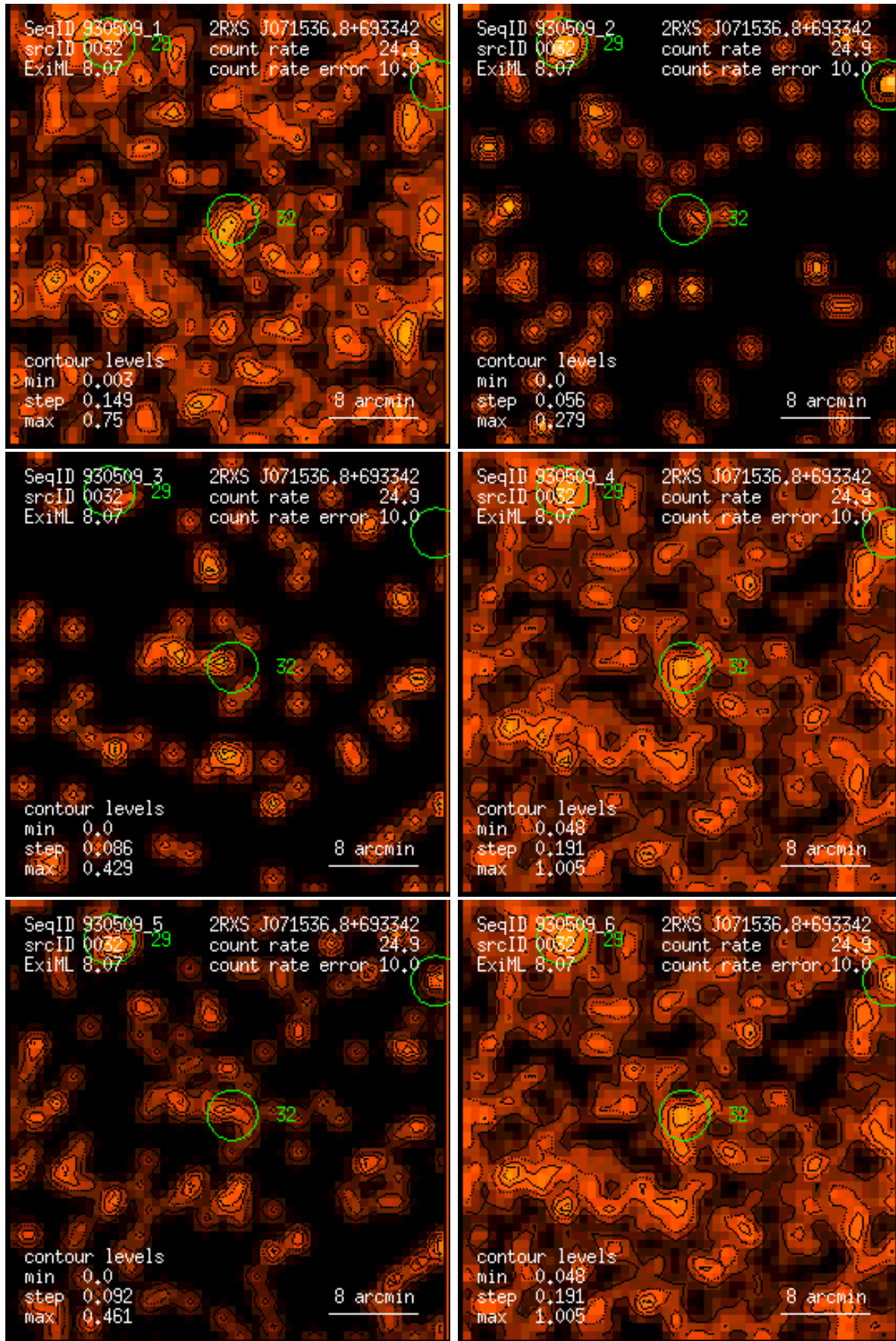
Figure 32: RASS 930509: detection 0032: band rate images, Gaussian filter: (1) PSPC channels 11 – 41, (2) 52 – 90, (3) 91 – 201, (4) 11 – 235, (5) 52 – 201, (6) 11 – 201. Broad band rates in counts/ks. Band rate contour levels in counts/ks/arcmin 2 .
