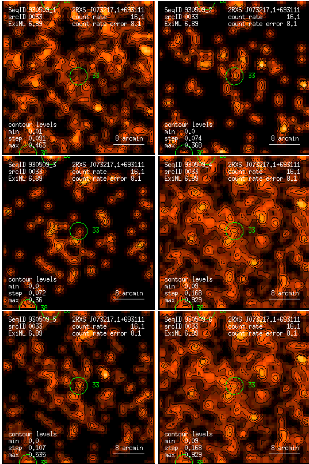
Figure 33: RASS 930509: detection 0033: band rate images, Gaussian filter: (1) PSPC channels 11 – 41, (2) 52 – 90, (3) 91 – 201, (4) 11 – 235, (5) 52 – 201, (6) 11 – 201. Broad band rates in counts/ks. Band rate contour levels in counts/ks/arcmin 2 .
