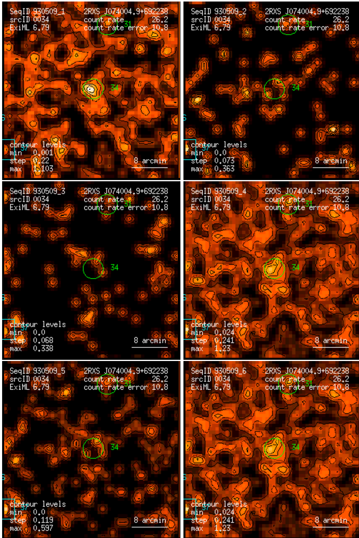
Figure 34: RASS 930509: detection 0034: band rate images, Gaussian filter: (1) PSPC channels 11 – 41, (2) 52 – 90, (3) 91 – 201, (4) 11 – 235, (5) 52 – 201, (6) 11 – 201. Broad band rates in counts/ks. Band rate contour levels in counts/ks/arcmin 2 .
