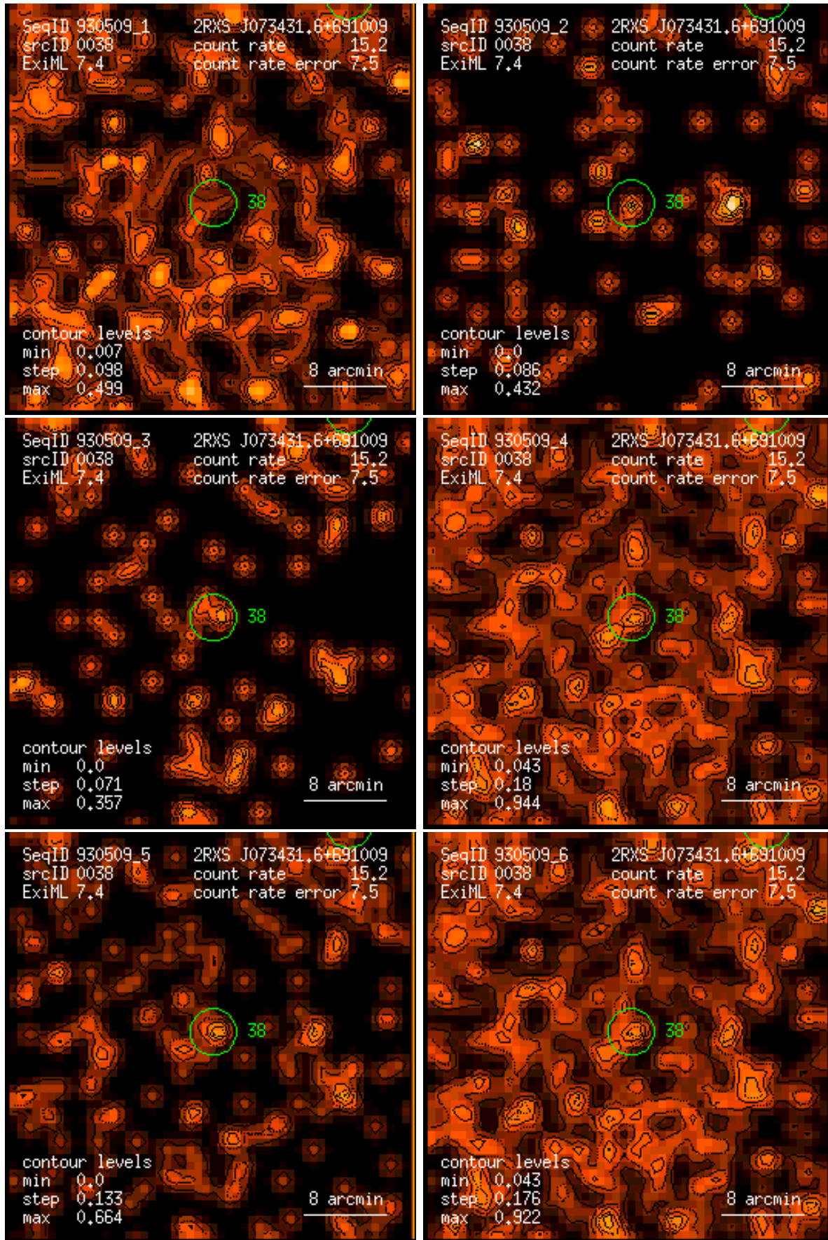
Figure 38: RASS 930509: detection 0038: band rate images, Gaussian filter: (1) PSPC channels 11 – 41, (2) 52 – 90, (3) 91 – 201, (4) 11 – 235, (5) 52 – 201, (6) 11 – 201. Broad band rates in counts/ks. Band rate contour levels in counts/ks/arcmin 2 .
