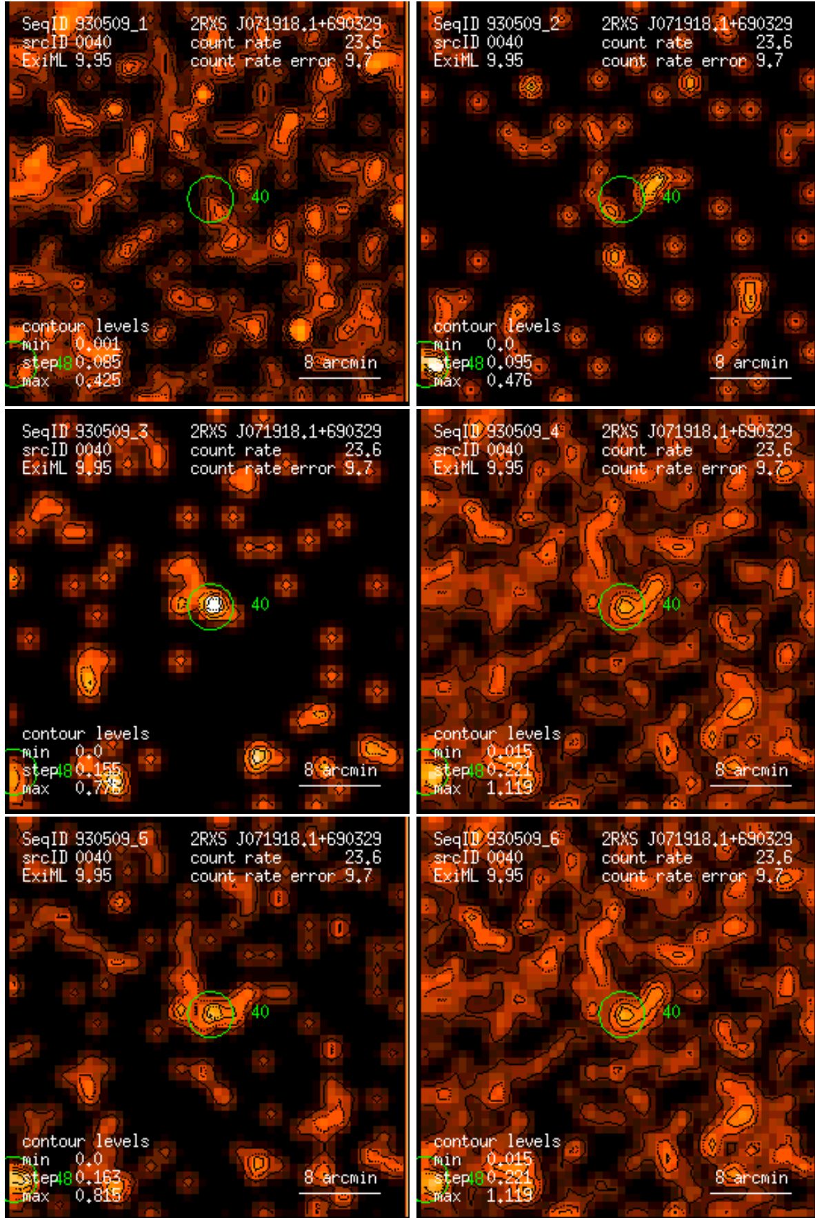
Figure 40: RASS 930509: detection 0040: band rate images, Gaussian filter: (1) PSPC channels 11 – 41, (2) 52 – 90, (3) 91 – 201, (4) 11 – 235, (5) 52 – 201, (6) 11 – 201. Broad band rates in counts/ks. Band rate contour levels in counts/ks/arcmin 2 .
