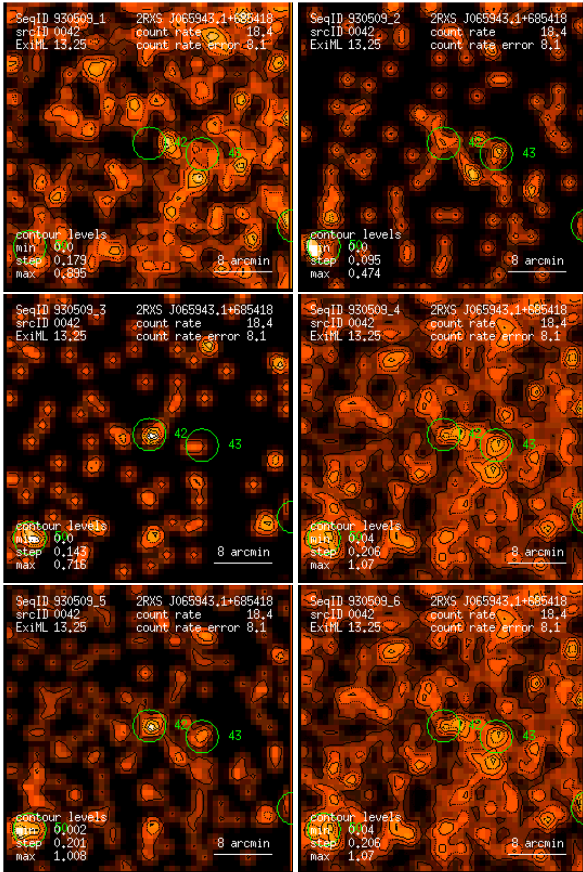
Figure 42: RASS 930509: detection 0042: band rate images, Gaussian filter: (1) PSPC channels 11 – 41, (2) 52 – 90, (3) 91 – 201, (4) 11 – 235, (5) 52 – 201, (6) 11 – 201. Broad band rates in counts/ks. Band rate contour levels in counts/ks/arcmin 2 .
