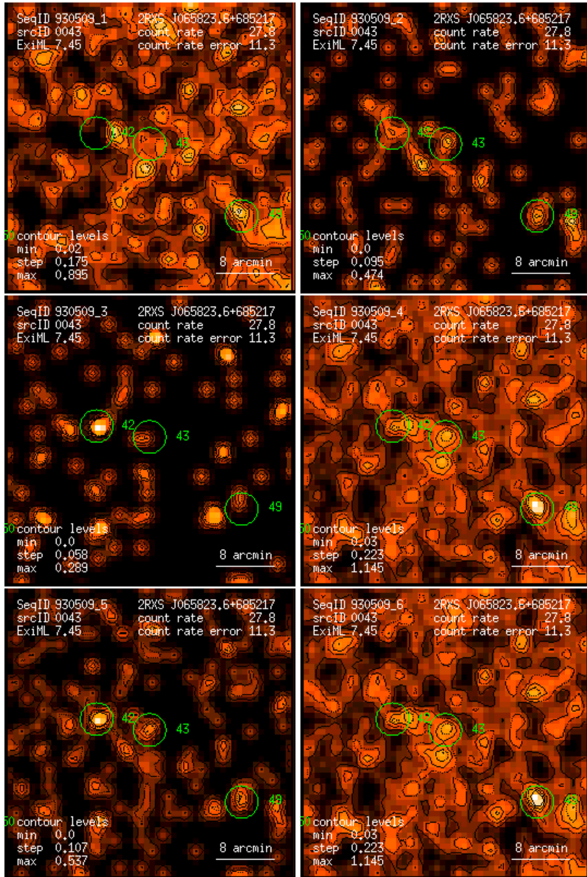
Figure 43: RASS 930509: detection 0043: band rate images, Gaussian filter: (1) PSPC channels 11 – 41, (2) 52 – 90, (3) 91 – 201, (4) 11 – 235, (5) 52 – 201, (6) 11 – 201. Broad band rates in counts/ks. Band rate contour levels in counts/ks/arcmin 2 .
