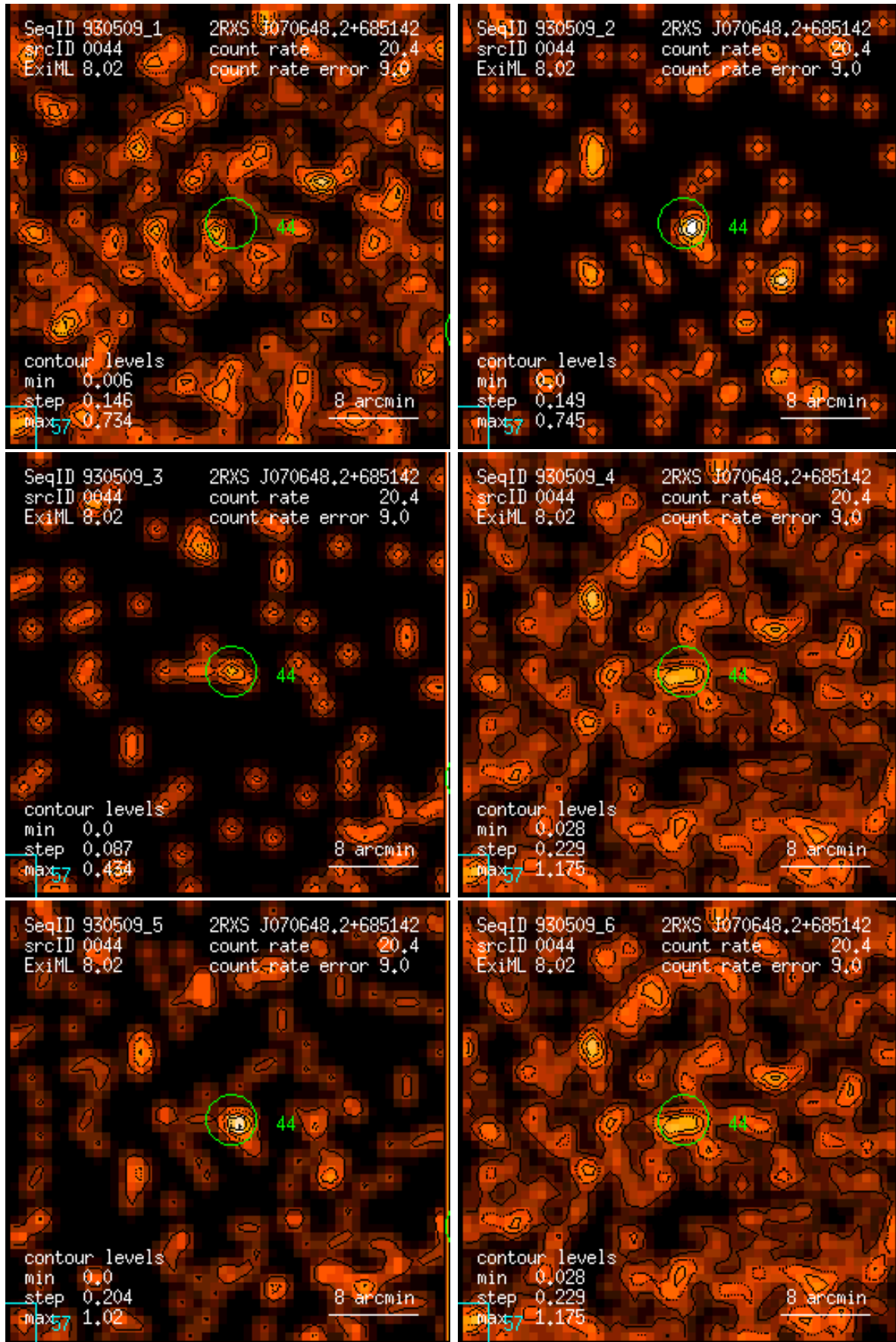
Figure 44: RASS 930509: detection 0044: band rate images, Gaussian filter: (1) PSPC channels 11 – 41, (2) 52 – 90, (3) 91 – 201, (4) 11 – 235, (5) 52 – 201, (6) 11 – 201. Broad band rates in counts/ks. Band rate contour levels in counts/ks/arcmin 2 .
