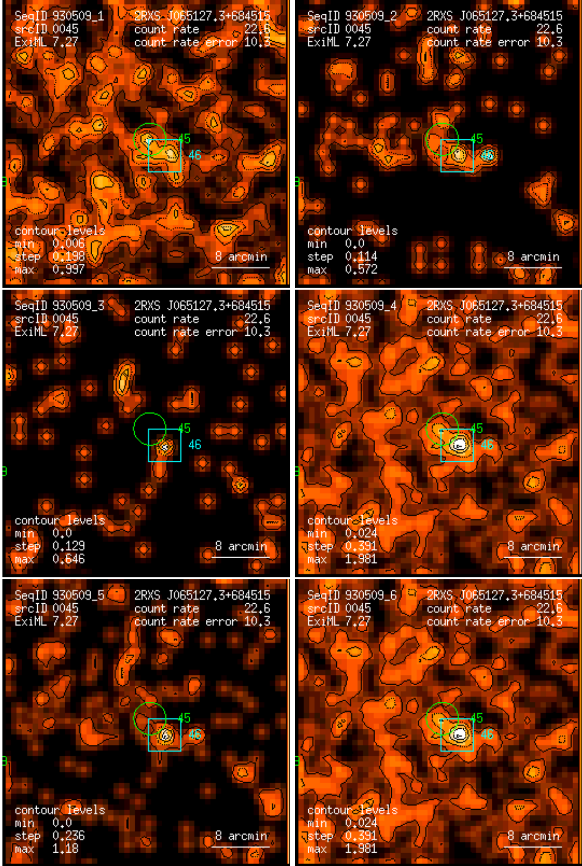
Figure 45: RASS 930509: detection 0045: band rate images, Gaussian filter: (1) PSPC channels 11 – 41, (2) 52 – 90, (3) 91 – 201, (4) 11 – 235, (5) 52 – 201, (6) 11 – 201. Broad band rates in counts/ks. Band rate contour levels in counts/ks/arcmin 2 .
