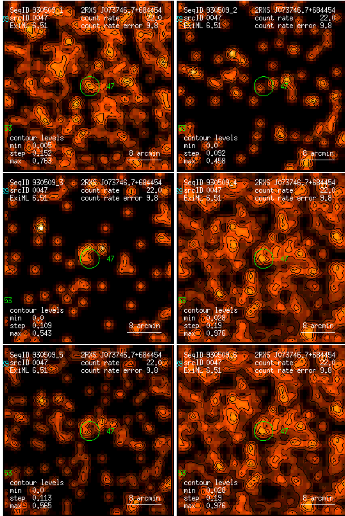
Figure 47: RASS 930509: detection 0047: band rate images, Gaussian filter: (1) PSPC channels 11 – 41, (2) 52 – 90, (3) 91 – 201, (4) 11 – 235, (5) 52 – 201, (6) 11 – 201. Broad band rates in counts/ks. Band rate contour levels in counts/ks/arcmin 2 .
