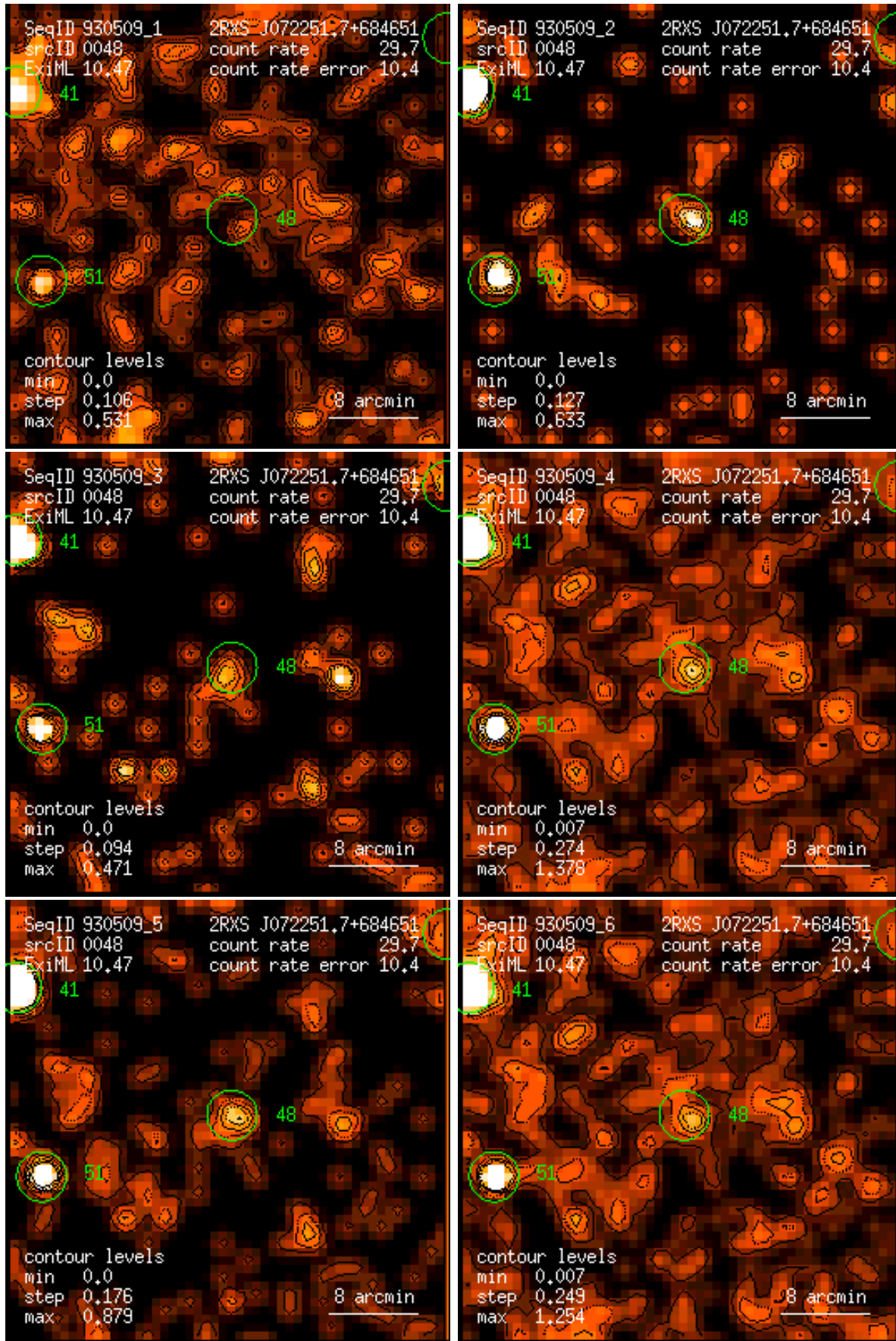
Figure 48: RASS 930509: detection 0048: band rate images, Gaussian filter: (1) PSPC channels 11 – 41, (2) 52 – 90, (3) 91 – 201, (4) 11 – 235, (5) 52 – 201, (6) 11 – 201. Broad band rates in counts/ks. Band rate contour levels in counts/ks/arcmin 2 .
