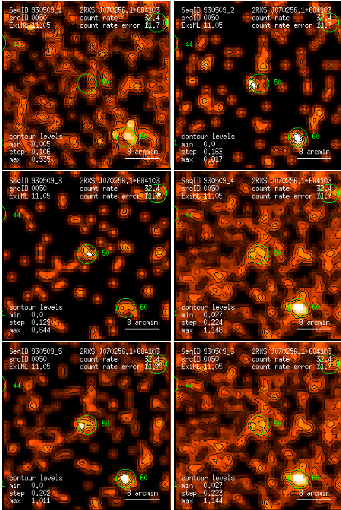
Figure 50: RASS 930509: detection 0050: band rate images, Gaussian filter: (1) PSPC channels 11 – 41, (2) 52 – 90, (3) 91 – 201, (4) 11 – 235, (5) 52 – 201, (6) 11 – 201. Broad band rates in counts/ks. Band rate contour levels in counts/ks/arcmin 2 .
