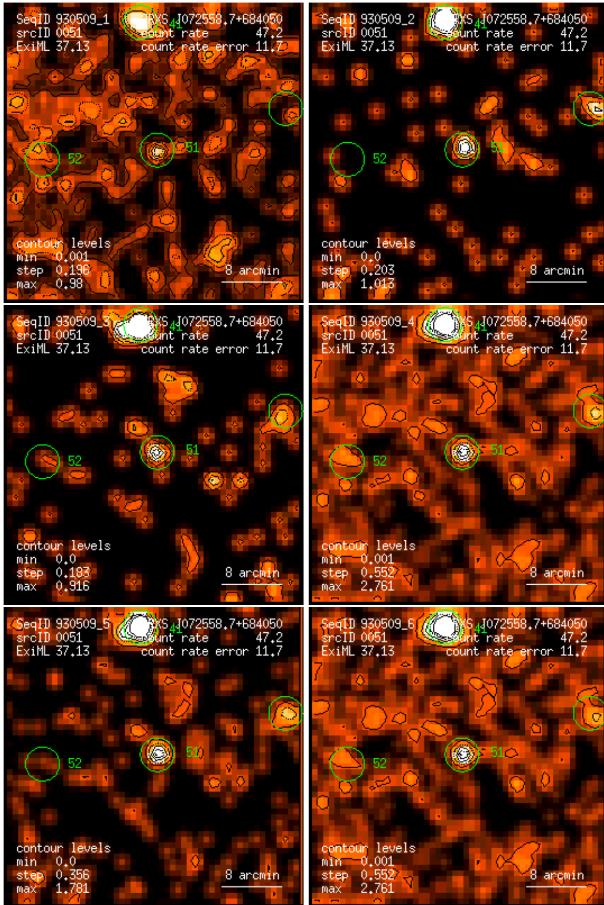
Figure 51: RASS 930509: detection 0051: band rate images, Gaussian filter: (1) PSPC channels 11 – 41, (2) 52 – 90, (3) 91 – 201, (4) 11 – 235, (5) 52 – 201, (6) 11 – 201. Broad band rates in counts/ks. Band rate contour levels in counts/ks/arcmin 2 .
