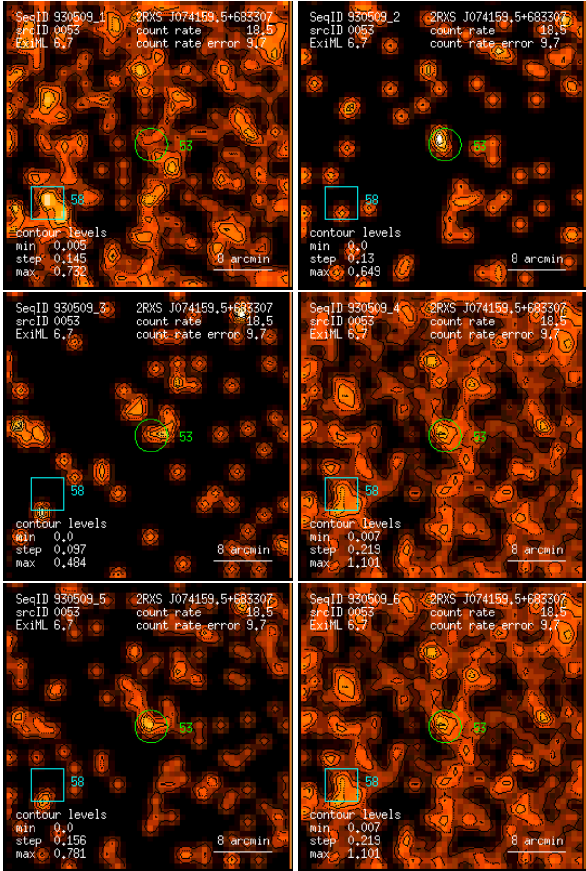
Figure 53: RASS 930509: detection 0053: band rate images, Gaussian filter: (1) PSPC channels 11 – 41, (2) 52 – 90, (3) 91 – 201, (4) 11 – 235, (5) 52 – 201, (6) 11 – 201. Broad band rates in counts/ks. Band rate contour levels in counts/ks/arcmin 2 .
