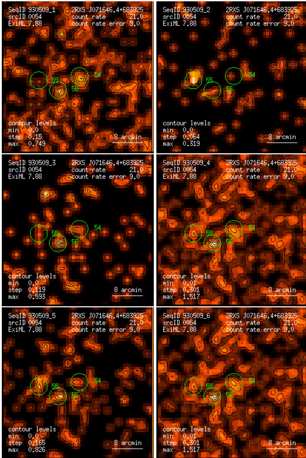
Figure 54: RASS 930509: detection 0054: band rate images, Gaussian filter: (1) PSPC channels 11 – 41, (2) 52 – 90, (3) 91 – 201, (4) 11 – 235, (5) 52 – 201, (6) 11 – 201. Broad band rates in counts/ks. Band rate contour levels in counts/ks/arcmin 2 .
