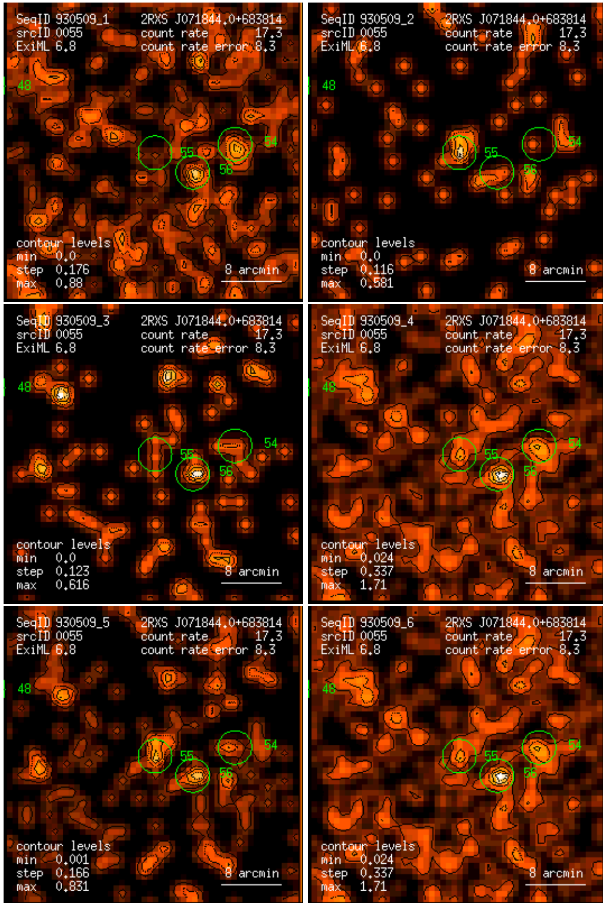
Figure 55: RASS 930509: detection 0055: band rate images, Gaussian filter: (1) PSPC channels 11 – 41, (2) 52 – 90, (3) 91 – 201, (4) 11 – 235, (5) 52 – 201, (6) 11 – 201. Broad band rates in counts/ks. Band rate contour levels in counts/ks/arcmin 2 .
