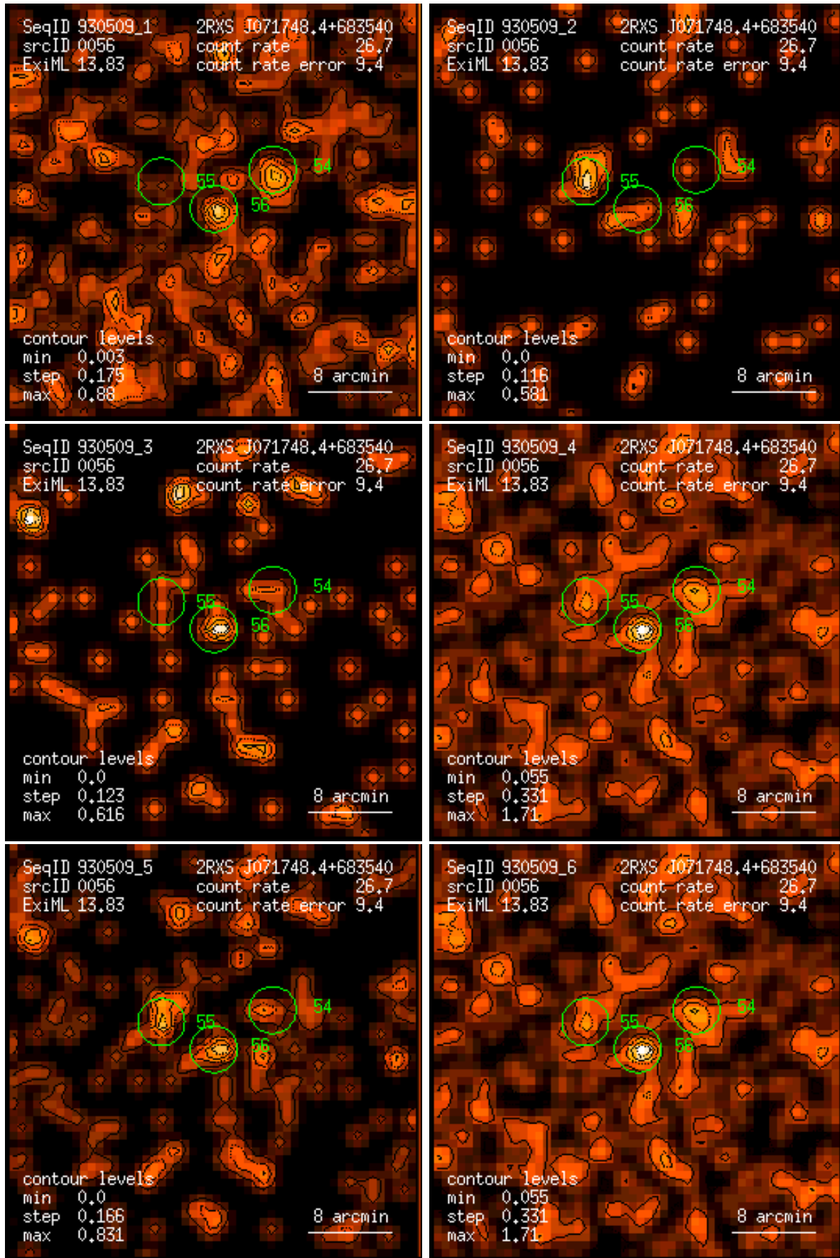
Figure 56: RASS 930509: detection 0056: band rate images, Gaussian filter: (1) PSPC channels 11 – 41, (2) 52 – 90, (3) 91 – 201, (4) 11 – 235, (5) 52 – 201, (6) 11 – 201. Broad band rates in counts/ks. Band rate contour levels in counts/ks/arcmin 2 .
