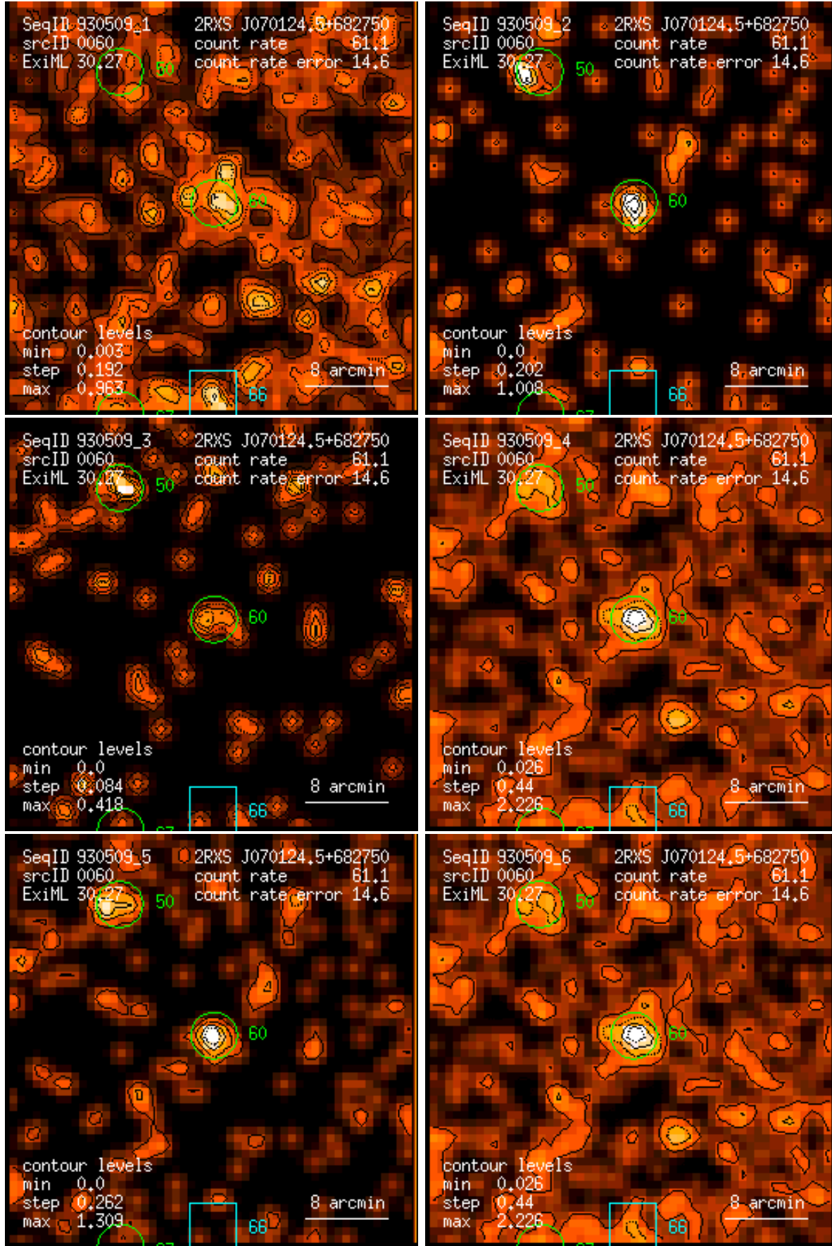
Figure 60: RASS 930509: detection 0060: band rate images, Gaussian filter: (1) PSPC channels 11 – 41, (2) 52 – 90, (3) 91 – 201, (4) 11 – 235, (5) 52 – 201, (6) 11 – 201. Broad band rates in counts/ks. Band rate contour levels in counts/ks/arcmin 2 .
