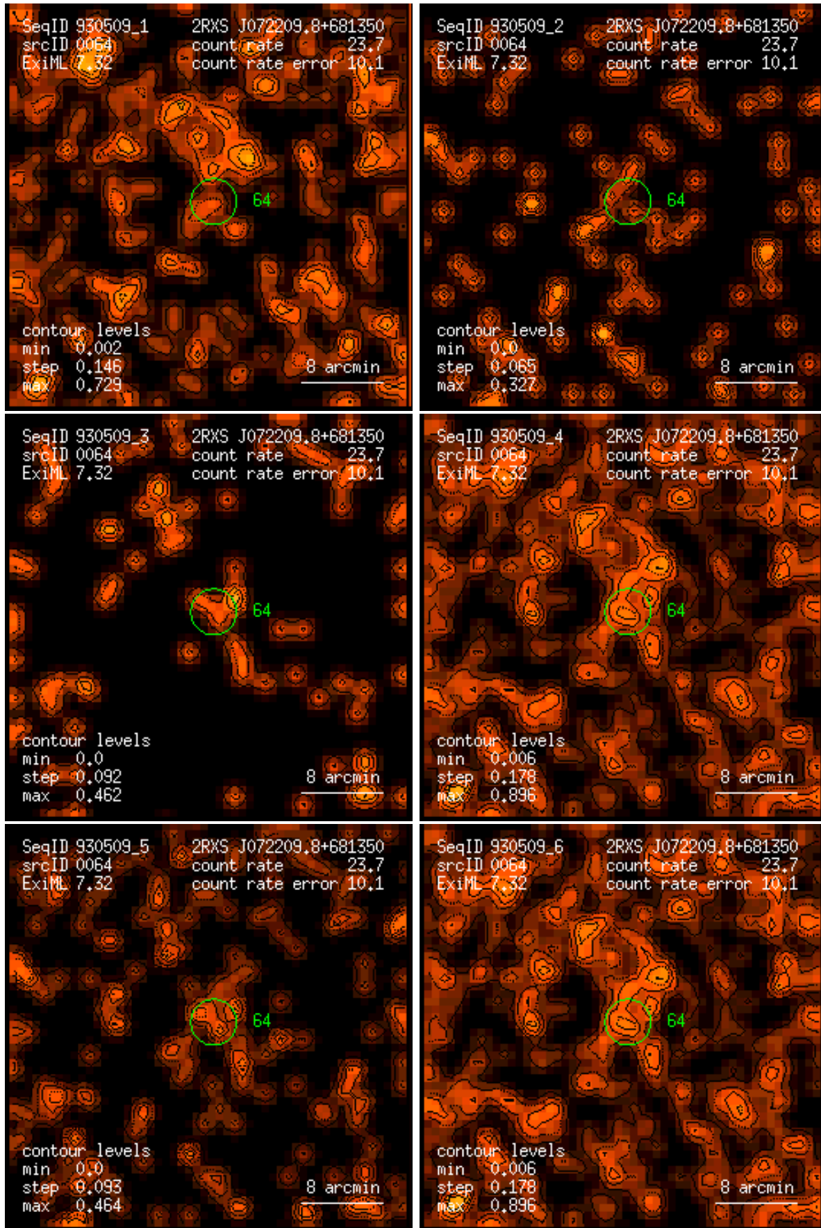
Figure 64: RASS 930509: detection 0064: band rate images, Gaussian filter: (1) PSPC channels 11 – 41, (2) 52 – 90, (3) 91 – 201, (4) 11 – 235, (5) 52 – 201, (6) 11 – 201. Broad band rates in counts/ks. Band rate contour levels in counts/ks/arcmin 2 .
