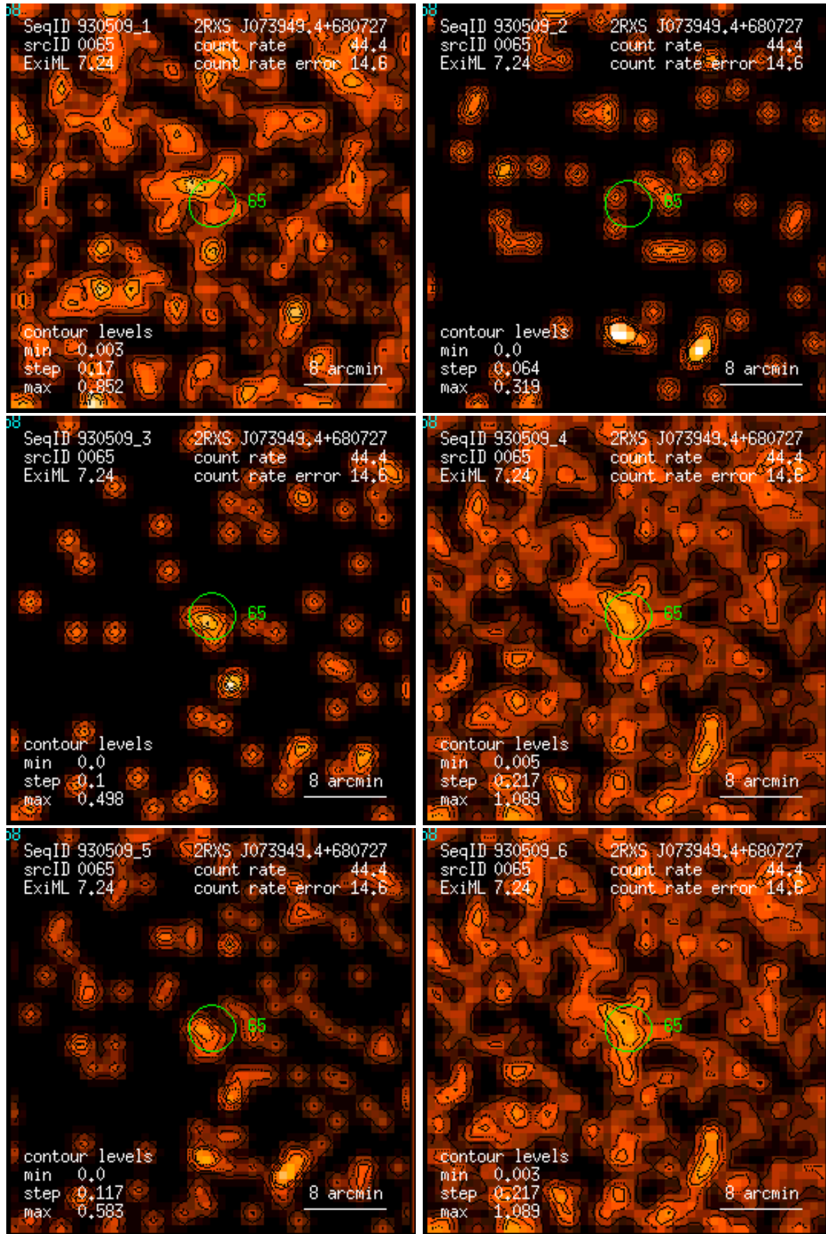
Figure 65: RASS 930509: detection 0065: band rate images, Gaussian filter: (1) PSPC channels 11 – 41, (2) 52 – 90, (3) 91 – 201, (4) 11 – 235, (5) 52 – 201, (6) 11 – 201. Broad band rates in counts/ks. Band rate contour levels in counts/ks/arcmin 2 .
