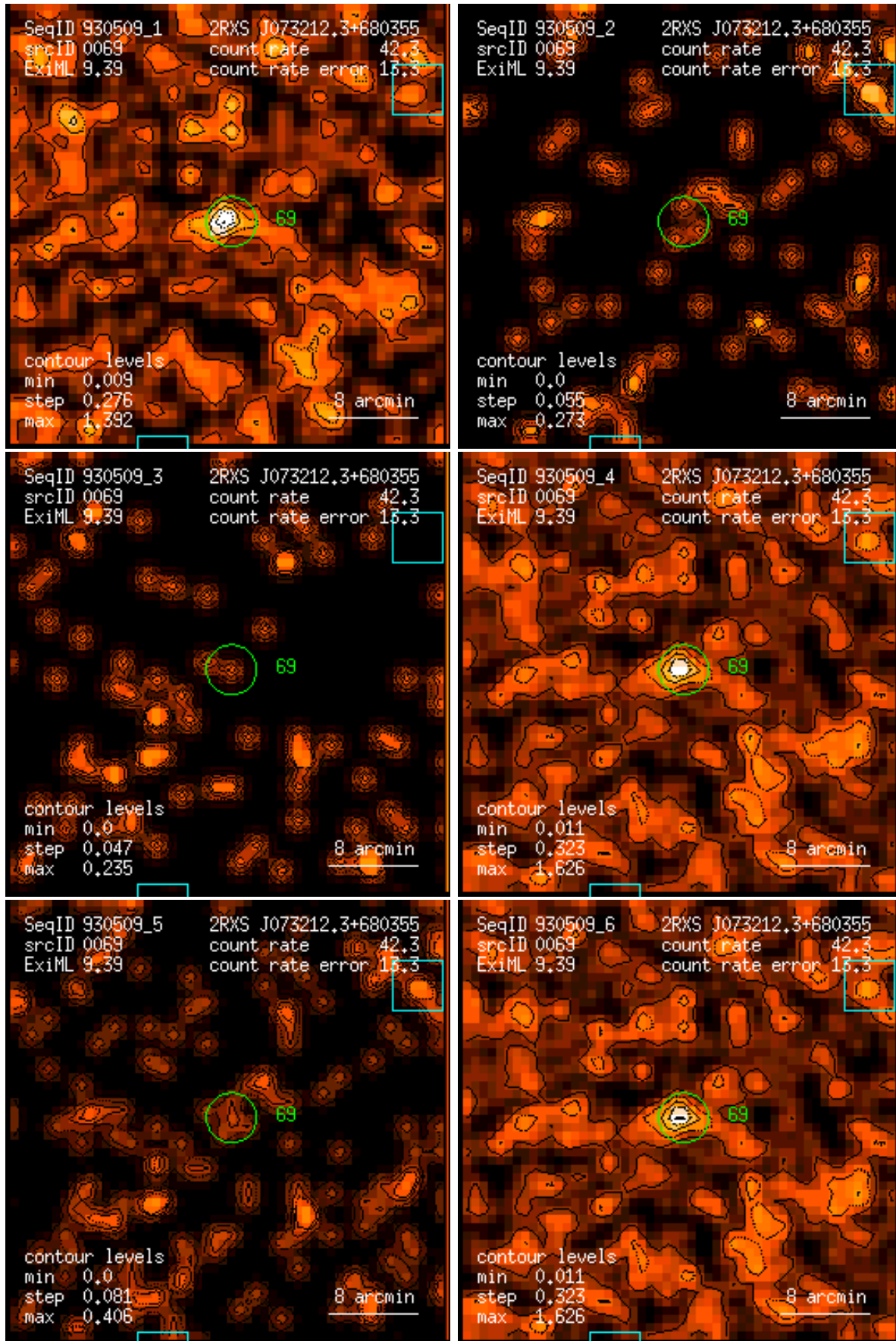
Figure 69: RASS 930509: detection 0069: band rate images, Gaussian filter: (1) PSPC channels 11 – 41, (2) 52 – 90, (3) 91 – 201, (4) 11 – 235, (5) 52 – 201, (6) 11 – 201. Broad band rates in counts/ks. Band rate contour levels in counts/ks/arcmin 2 .
