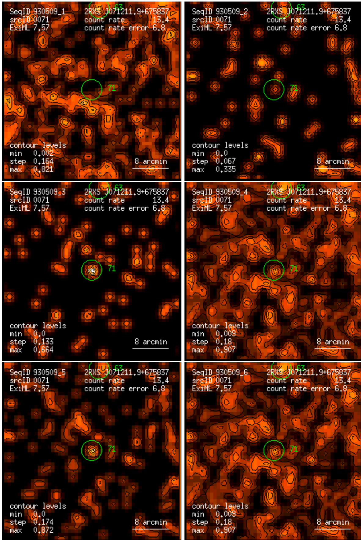
Figure 71: RASS 930509: detection 0071: band rate images, Gaussian filter: (1) PSPC channels 11 – 41, (2) 52 – 90, (3) 91 – 201, (4) 11 – 235, (5) 52 – 201, (6) 11 – 201. Broad band rates in counts/ks. Band rate contour levels in counts/ks/arcmin 2 .
