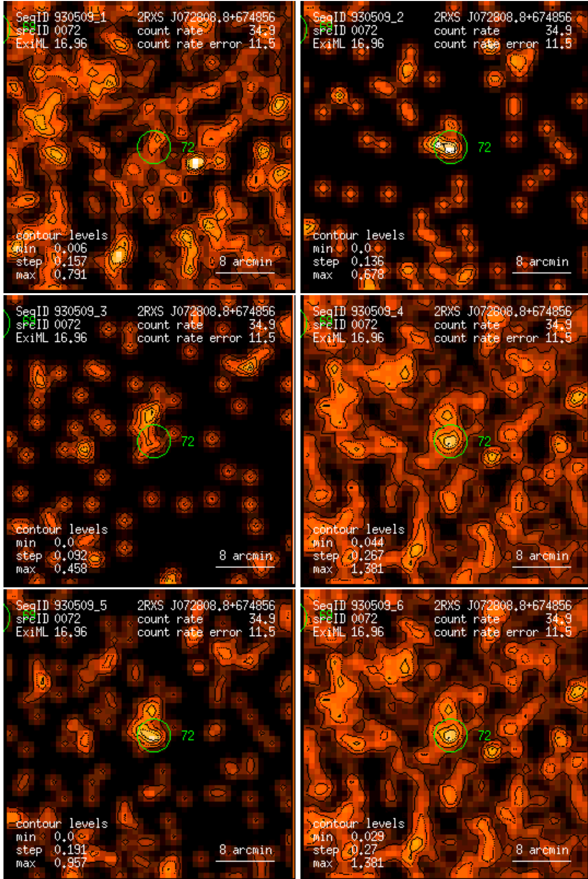
Figure 72: RASS 930509: detection 0072: band rate images, Gaussian filter: (1) PSPC channels 11 – 41, (2) 52 – 90, (3) 91 – 201, (4) 11 – 235, (5) 52 – 201, (6) 11 – 201. Broad band rates in counts/ks. Band rate contour levels in counts/ks/arcmin 2 .
