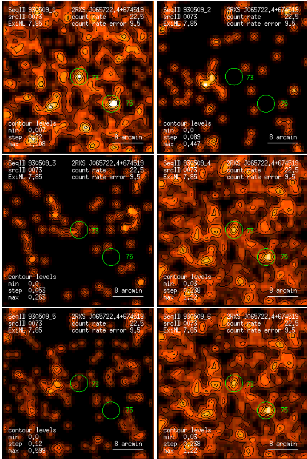
Figure 73: RASS 930509: detection 0073: band rate images, Gaussian filter: (1) PSPC channels 11 – 41, (2) 52 – 90, (3) 91 – 201, (4) 11 – 235, (5) 52 – 201, (6) 11 – 201. Broad band rates in counts/ks. Band rate contour levels in counts/ks/arcmin 2 .
